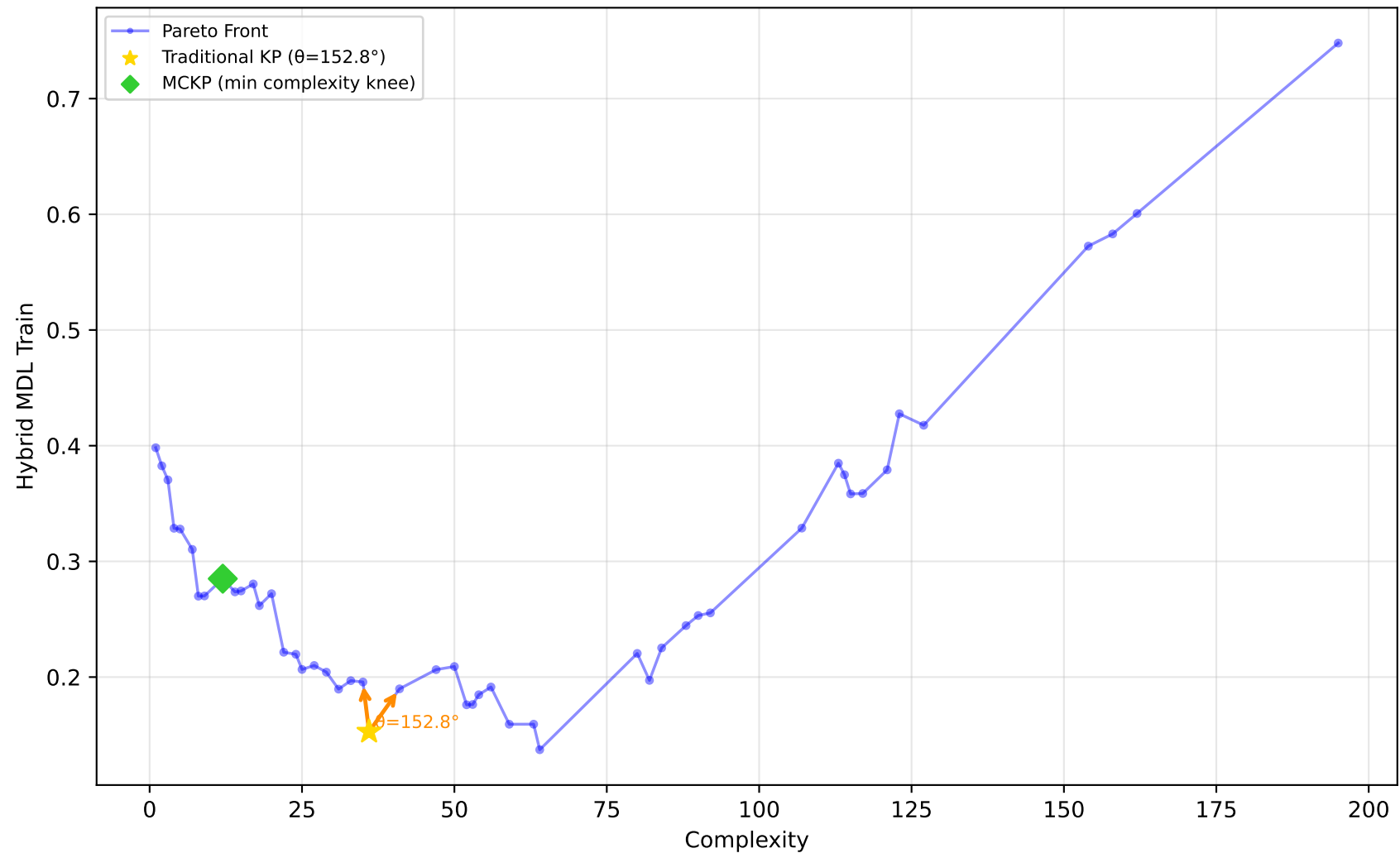
584_fri_c4_500_25 - Run 26 - SVP - Hybrid MDL Train \lambda_1=0.10, \lambda_2=0.40, \lambda_3=0.00 | Difficulty: 1.00 | Method: hmr
