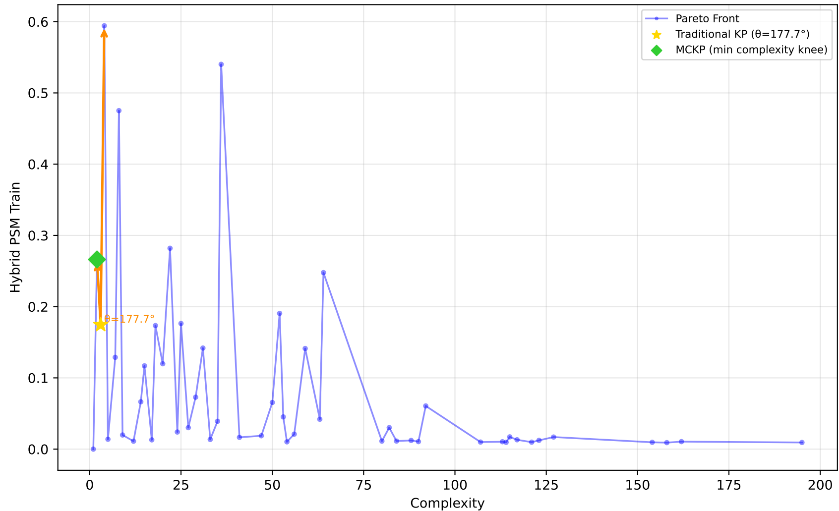
584_fri_c4_500_25 - Run 26 - SVP - Hybrid PSM Train \lambda_1=0.10, \lambda_2=0.40, \lambda_3=0.00 | Difficulty: 1.00 | Method: hmr
