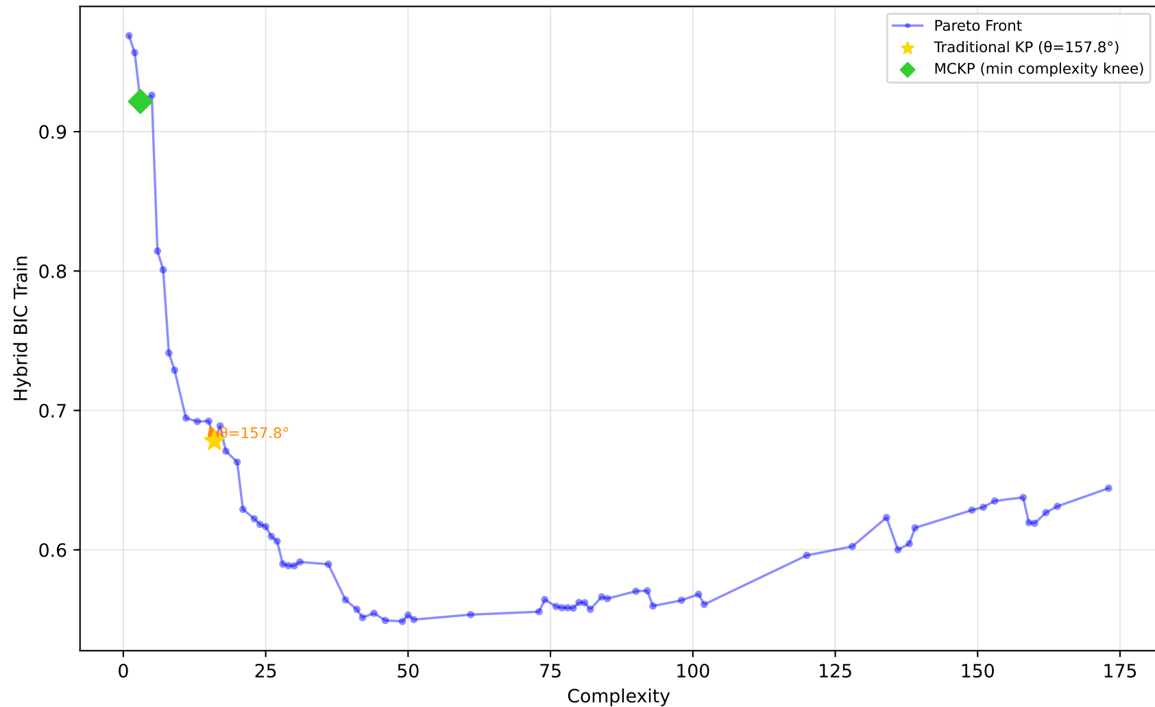
584_fri_c4_500_25 - Run 27 - MVP - Hybrid BIC Train \lambda_1=0.10, \lambda_2=0.00, \lambda_3=0.00 | Difficulty: 1.00 | Method: hmr
