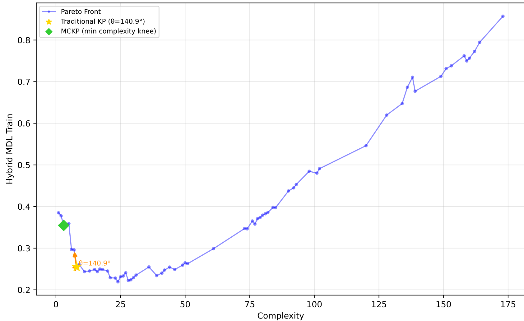
584_fri_c4_500_25 - Run 27 - MVP - Hybrid MDL Train \lambda_1=0.00, \bar{\lambda}_2=0.00, \bar{\lambda}_3=0.00 | Difficulty: 1.00 | Method: hmr
