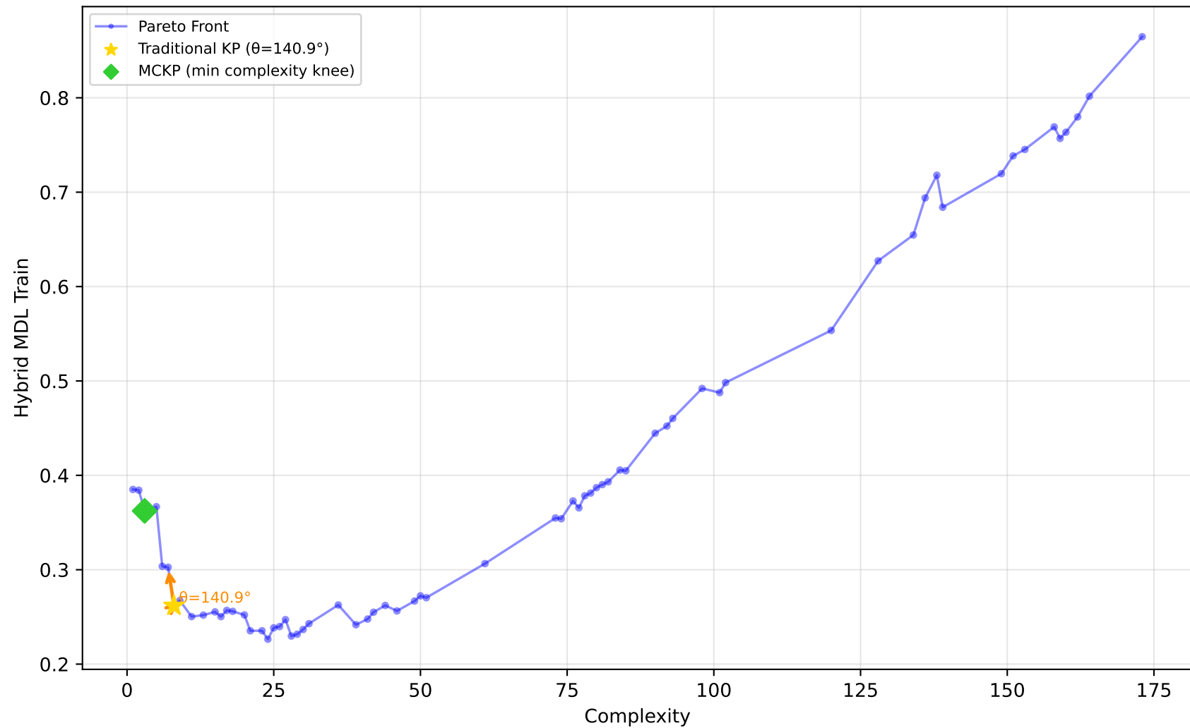
584_fri_c4_500_25 - Run 27 - MVP - Hybrid MDL Train \lambda_1=0.10, \bar{\lambda}_2=0.00, \bar{\lambda}_3=0.00 | Difficulty: 1.00 | Method: hmr
