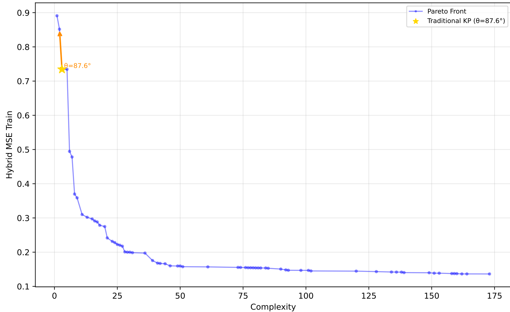
584_fri_c4_500_25 - Run 27 - MVP - Hybrid MSE Train \lambda_1=0.10, \bar{\lambda}_2=0.00, \bar{\lambda}_3=0.00 | Difficulty: 1.00 | Method: hmr
