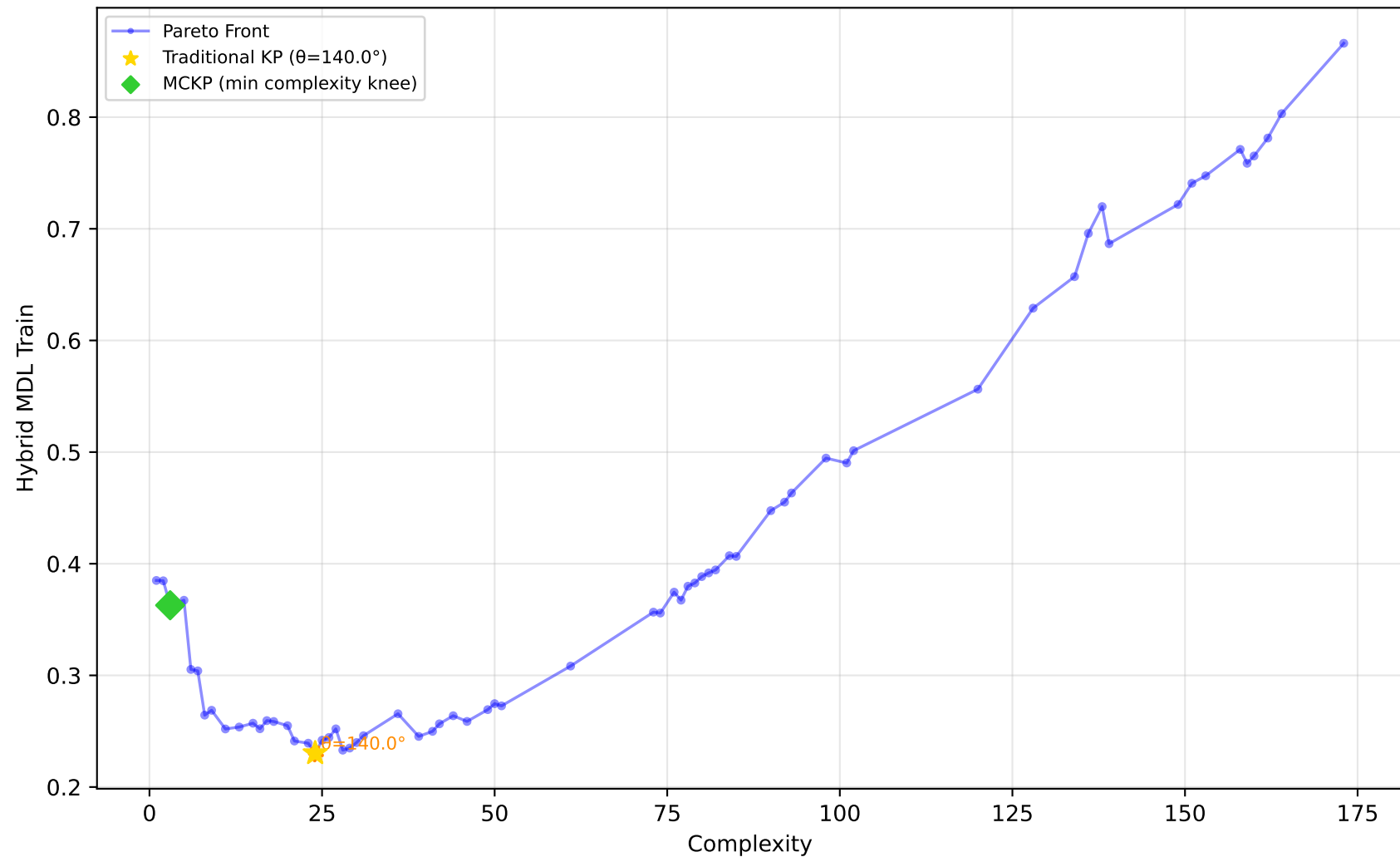
584_fri_c4_500_25 - Run 27 - SVP - Hybrid MDL Train \lambda_1=0.10, \lambda_2=0.40, \lambda_3=0.00 | Difficulty: 1.00 | Method: hmr
