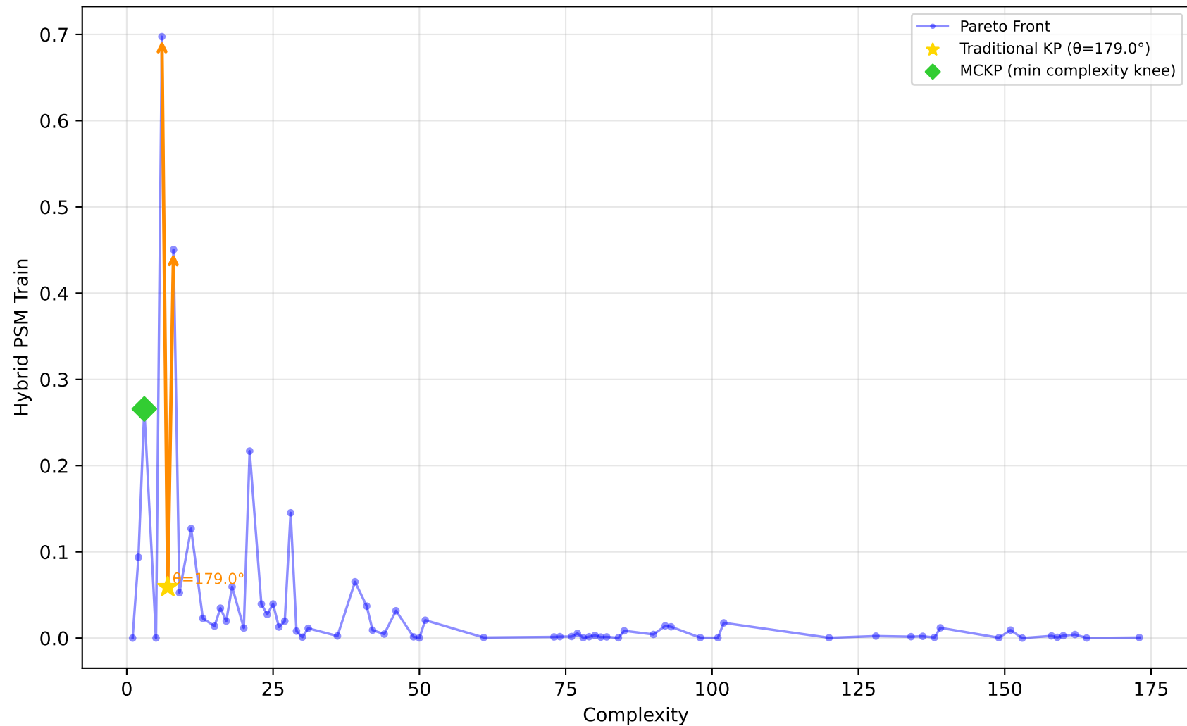
584_fri_c4_500_25 - Run 27 - SVP - Hybrid PSM Train \lambda_1=0.00, \lambda_2=0.00, \lambda_3=0.00 | Difficulty: 1.00 | Method: hmr
