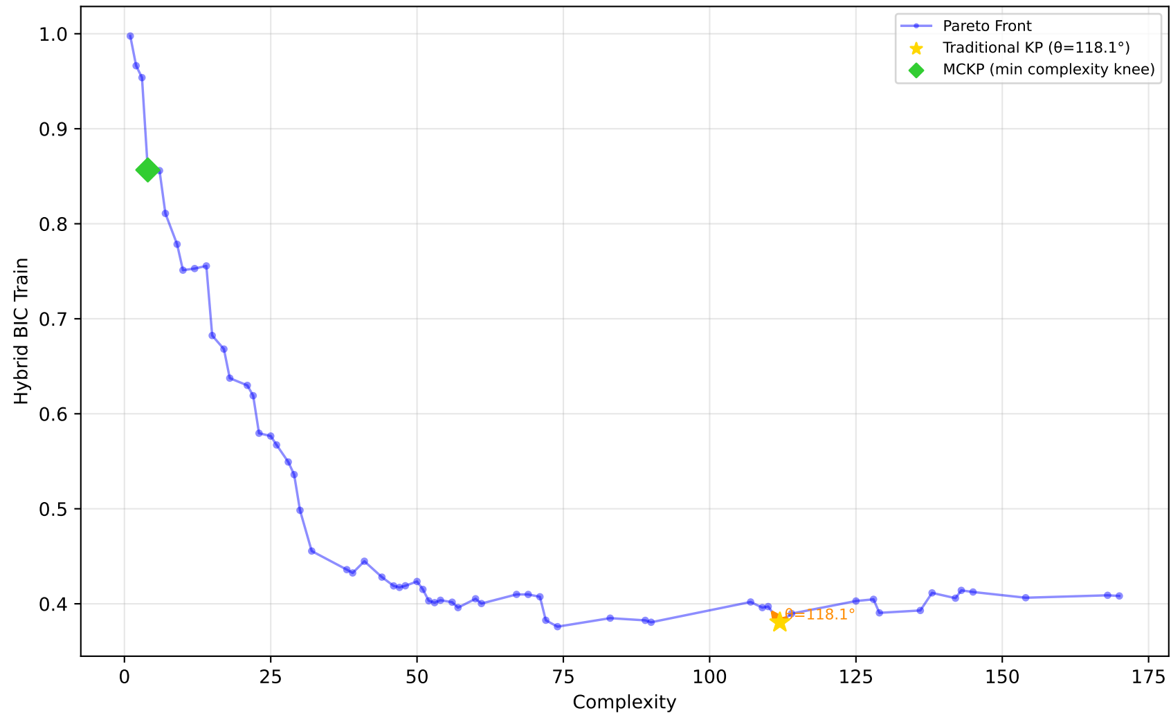
584_fri_c4_500_25 - Run 28 - SVP - Hybrid BIC Train \lambda_1=0.10, \lambda_2=0.40, \lambda_3=0.00 | Difficulty: 1.00 | Method: hmr
