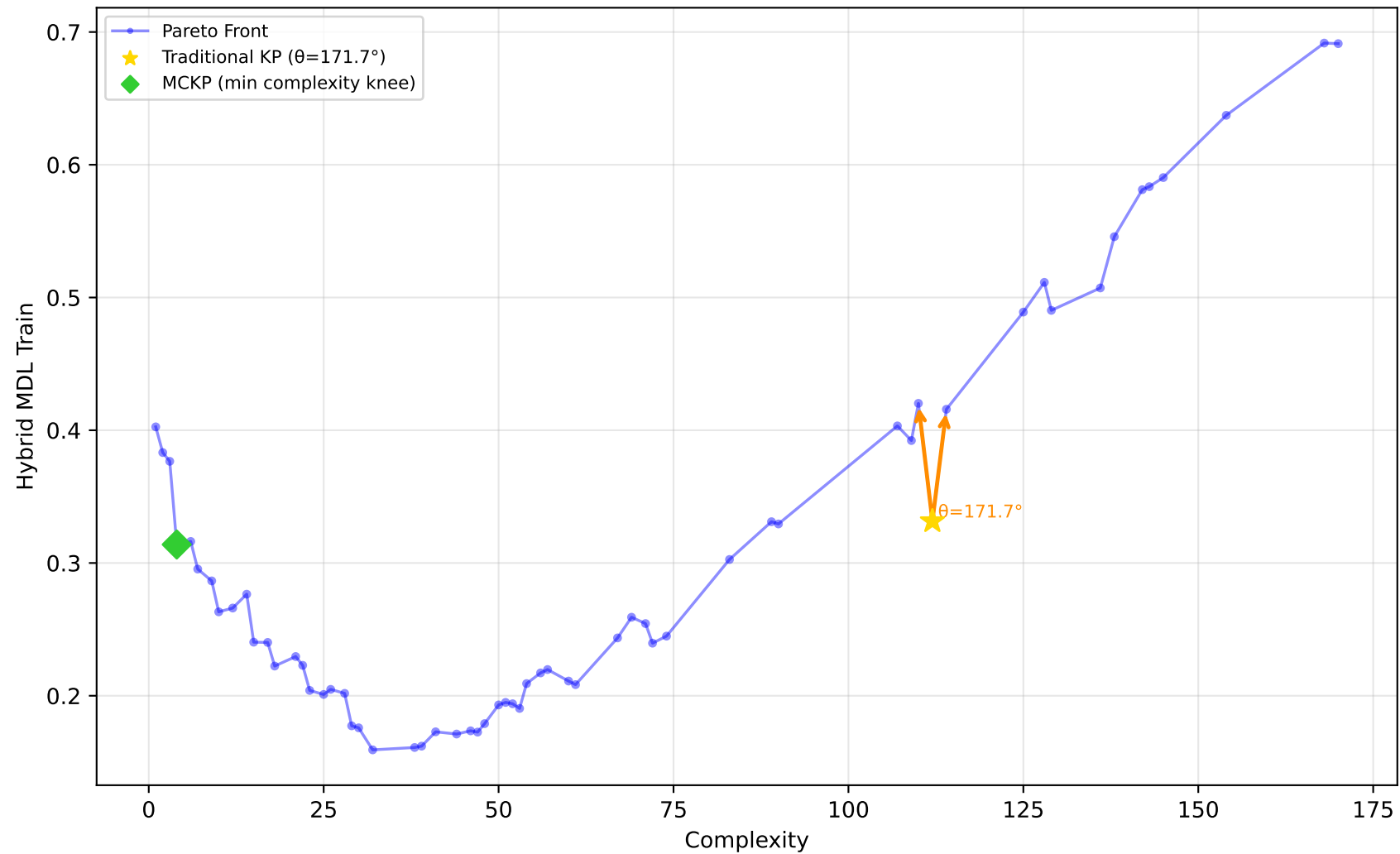
584_fri_c4_500_25 - Run 28 - SVP - Hybrid MDL Train \lambda_1=0.00, \bar{\lambda}_2=0.00, \bar{\lambda}_3=0.00 | Difficulty: 1.00 | Method: hmr
