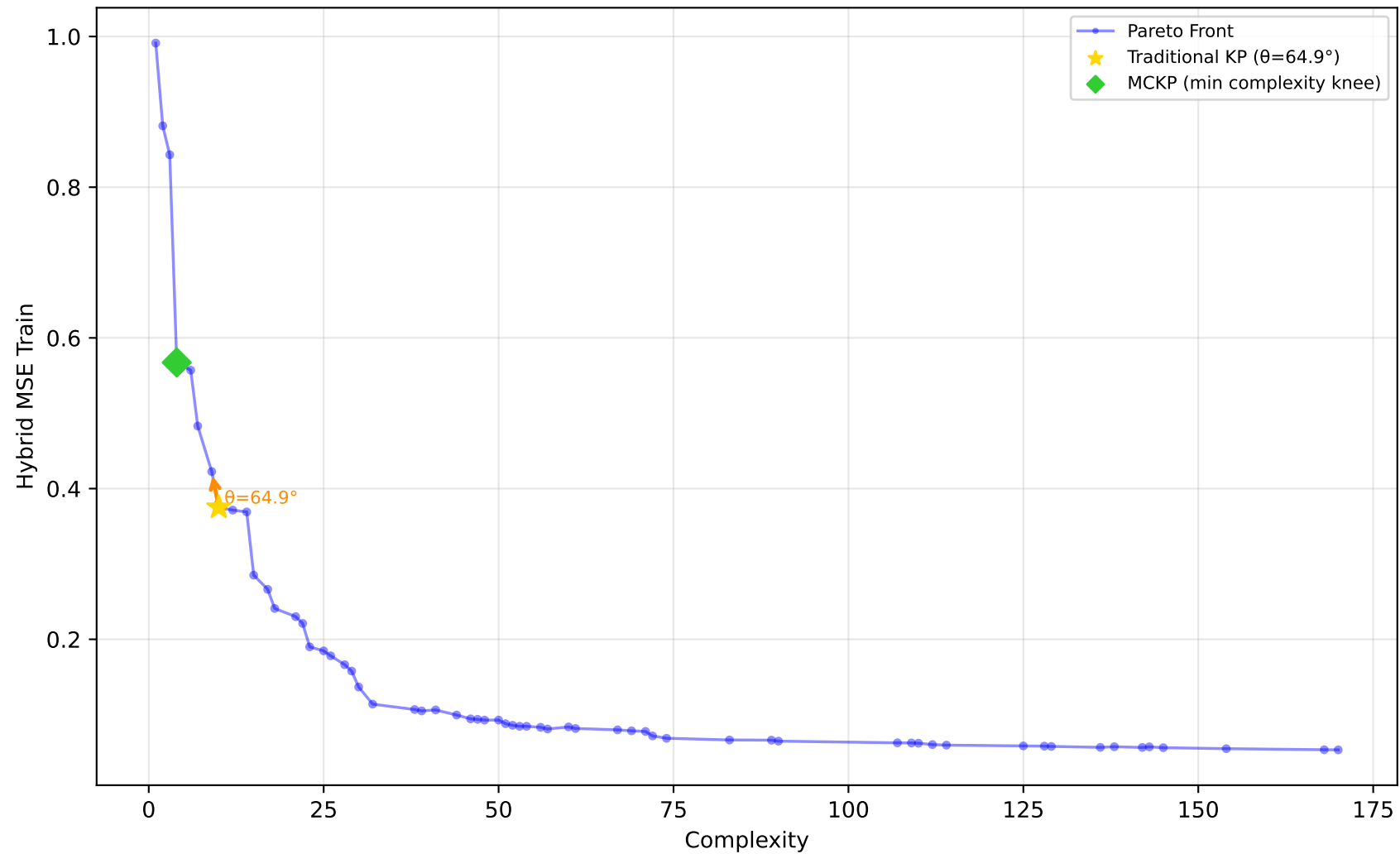
584_fri_c4_500_25 - Run 28 - SVP - Hybrid MSE Train \lambda_1=0.10, \lambda_2=0.40, \lambda_3=0.00 | Difficulty: 1.00 | Method: hmr
