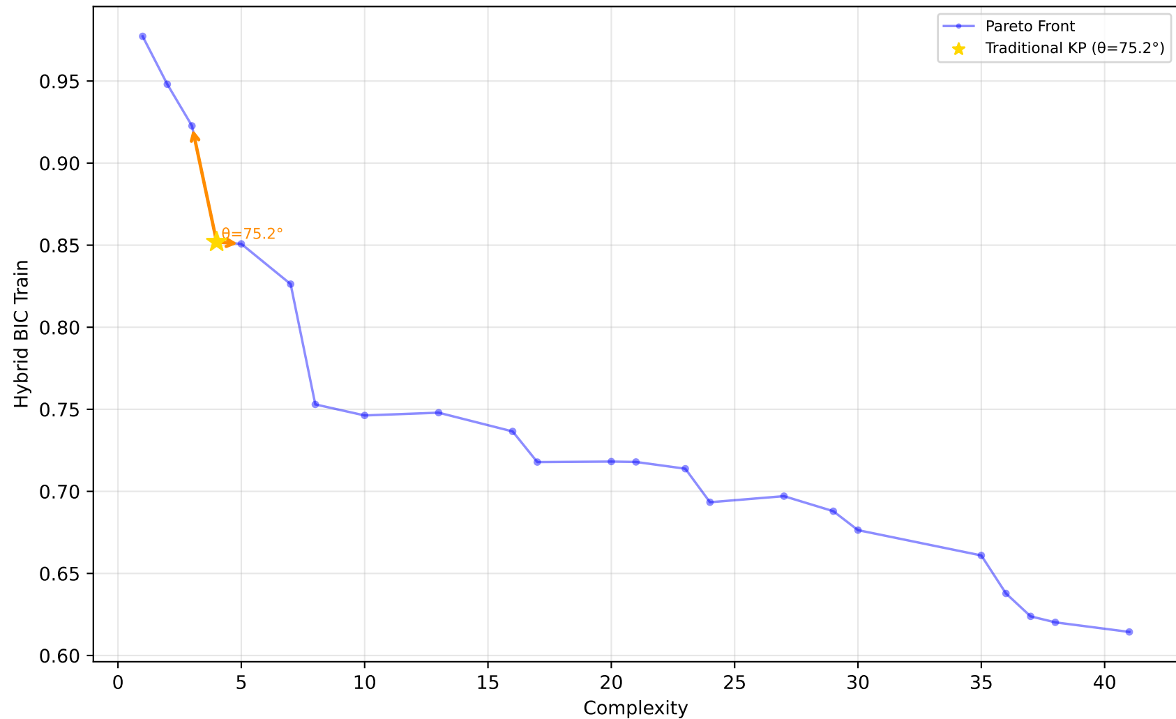
584_fri_c4_500_25 - Run 29 - MVP - Hybrid BIC Train \lambda_1=0.10, \lambda_2=0.00, \lambda_3=0.00 | Difficulty: 1.00 | Method: hmr
