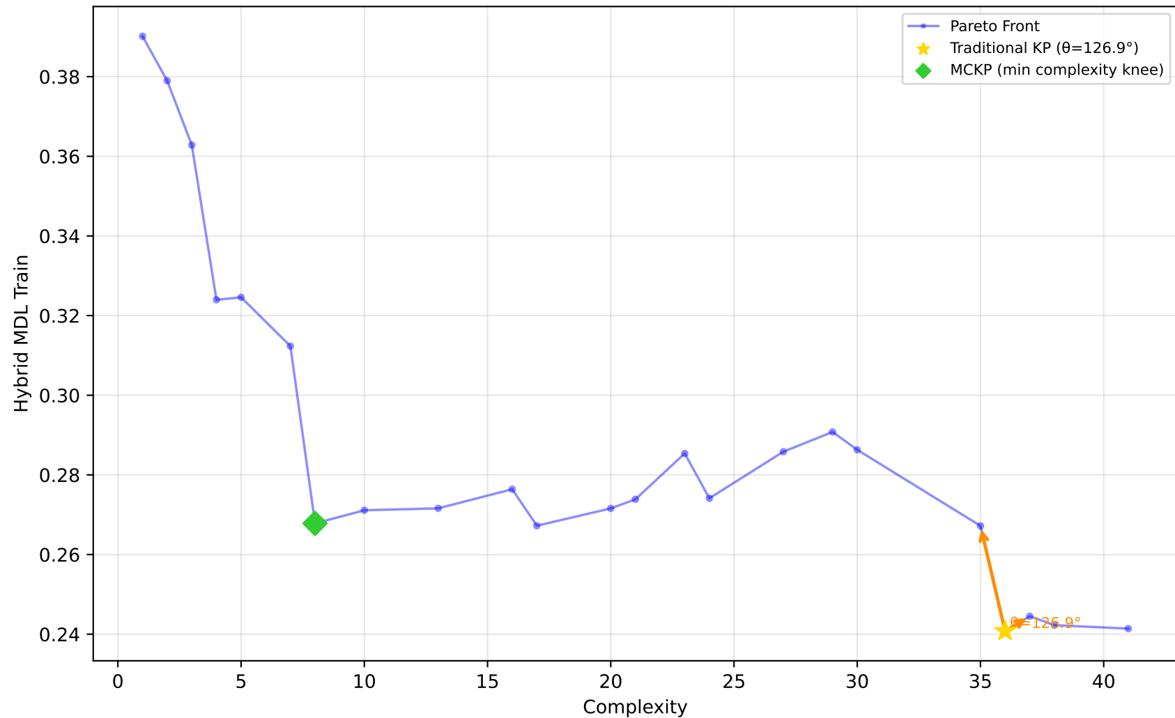
584_fri_c4_500_25 - Run 29 - MVP - Hybrid MDL Train \lambda_1=0.10, \lambda_2=0.00, \lambda_3=0.00 | Difficulty: 1.00 | Method: hmr
