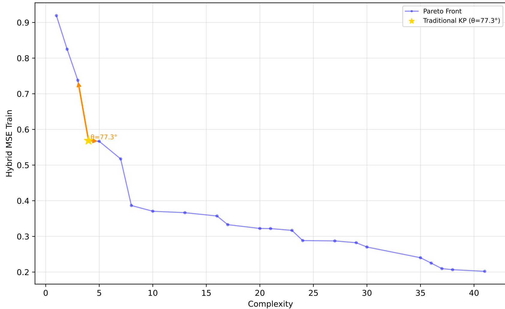
584_fri_c4_500_25 - Run 29 - MVP - Hybrid MSE Train \lambda_1=0.10, \lambda_2=0.00, \lambda_3=0.00 | Difficulty: 1.00 | Method: hmr
