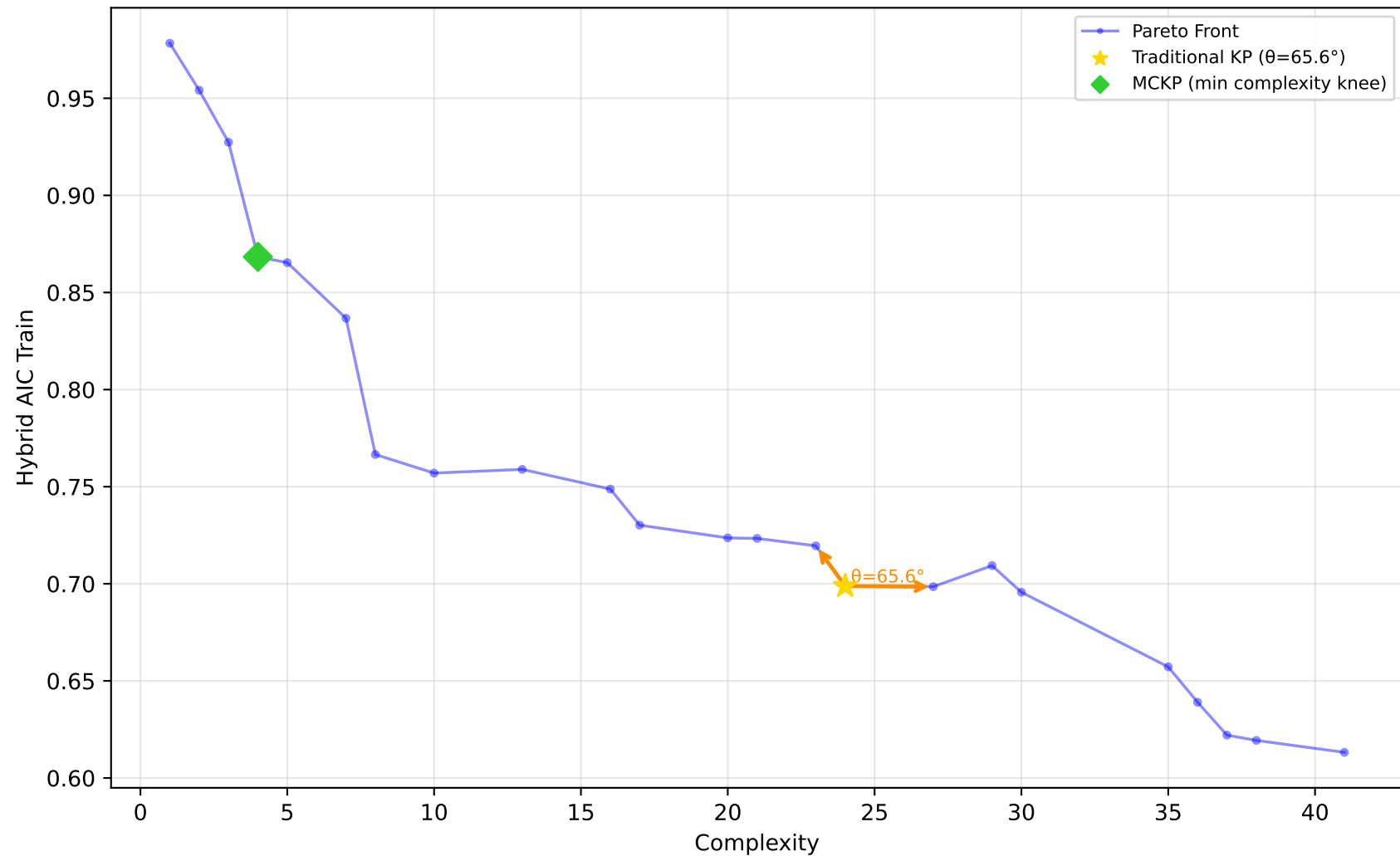
584_fri_c4_500_25 - Run 29 - SVP - Hybrid AIC Train \lambda_1=0.10, \lambda_2=0.40, \lambda_3=0.00 | Difficulty: 1.00 | Method: hmr
