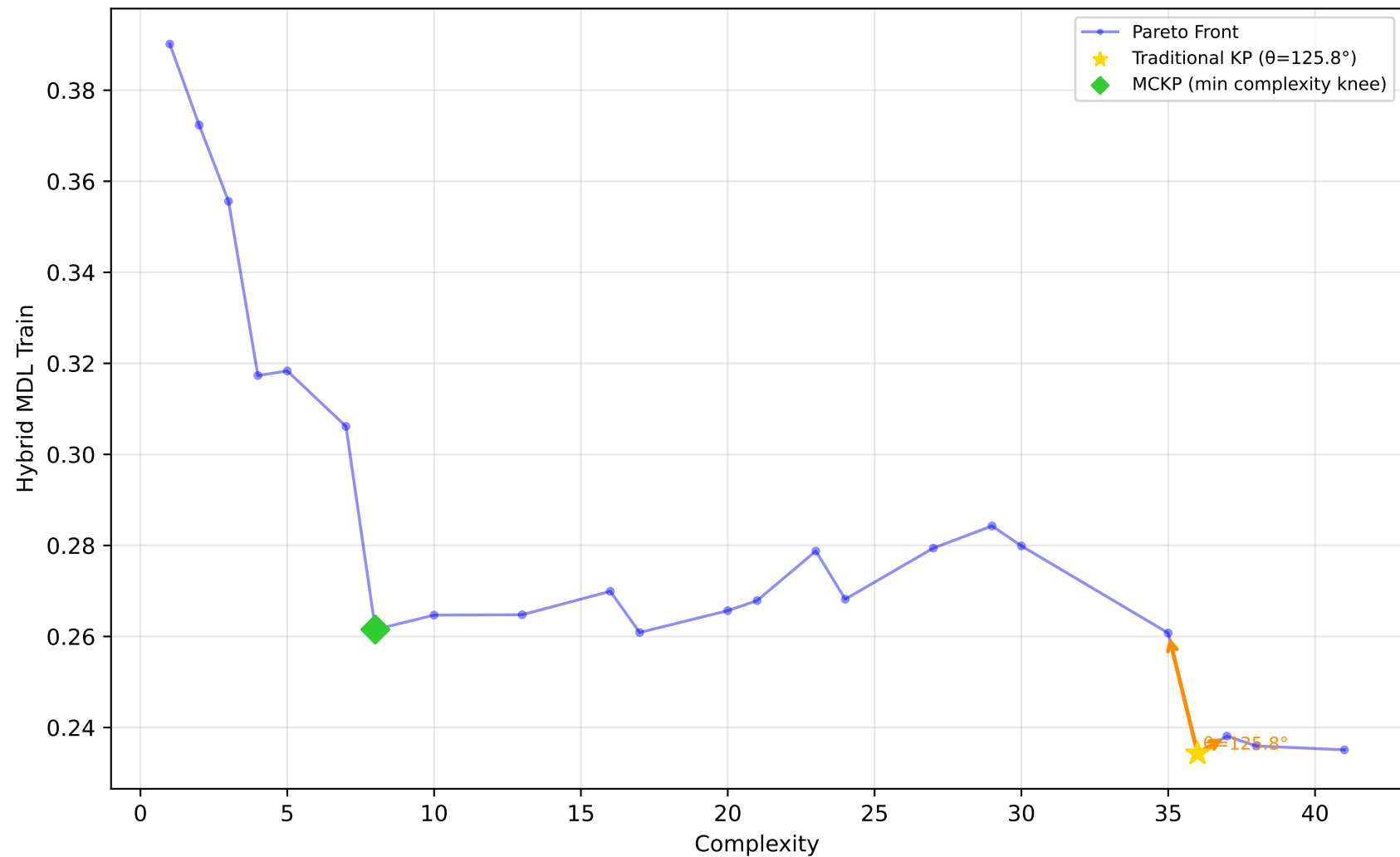
584_fri_c4_500_25 - Run 29 - SVP - Hybrid MDL Train \lambda_1=0.00, \lambda_2=0.00, \lambda_3=0.00 | Difficulty: 1.00 | Method: hmr
