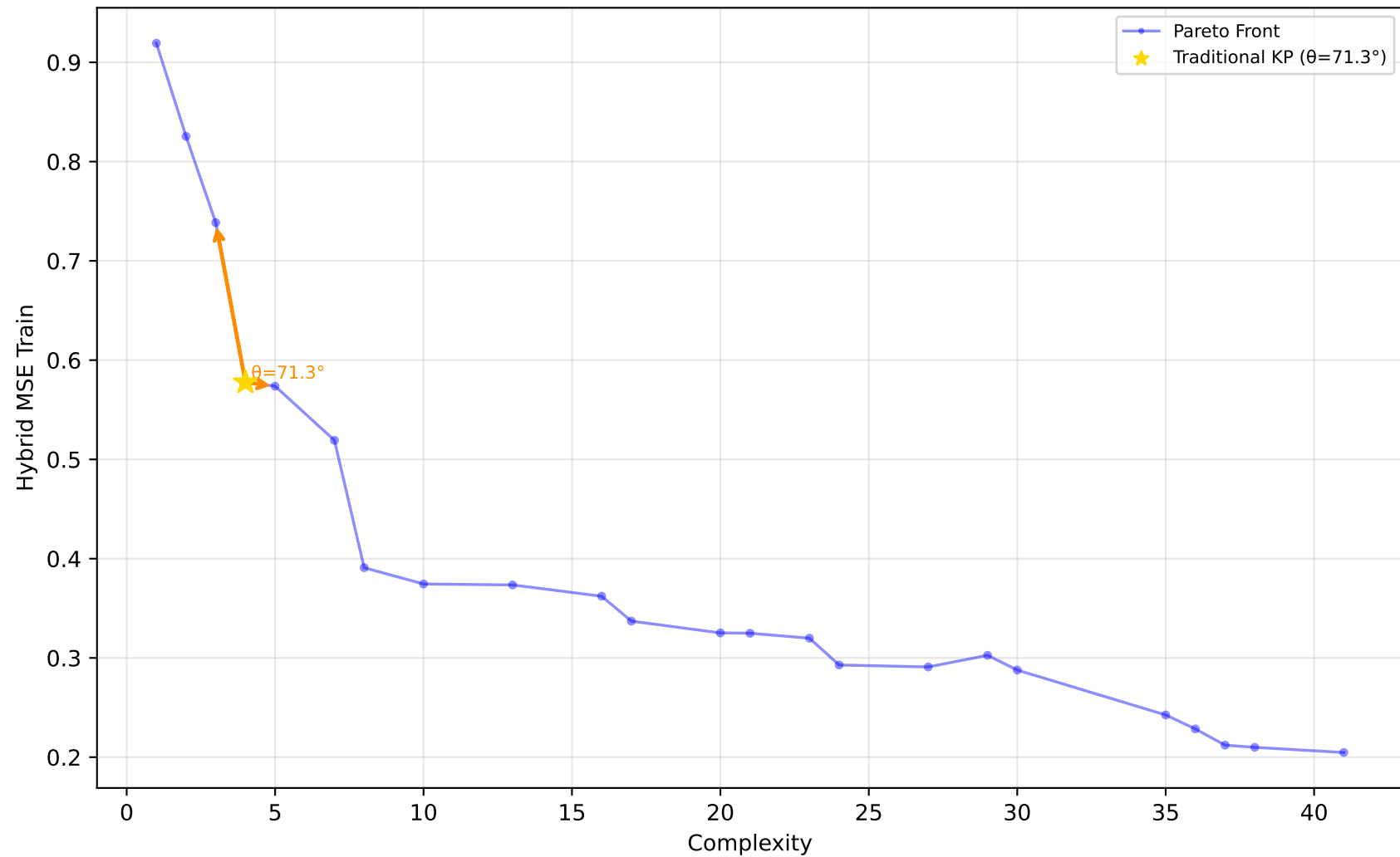
584_fri_c4_500_25 - Run 29 - SVP - Hybrid MSE Train \lambda_1=0.10, \lambda_2=0.40, \lambda_3=0.00 | Difficulty: 1.00 | Method: hmr
