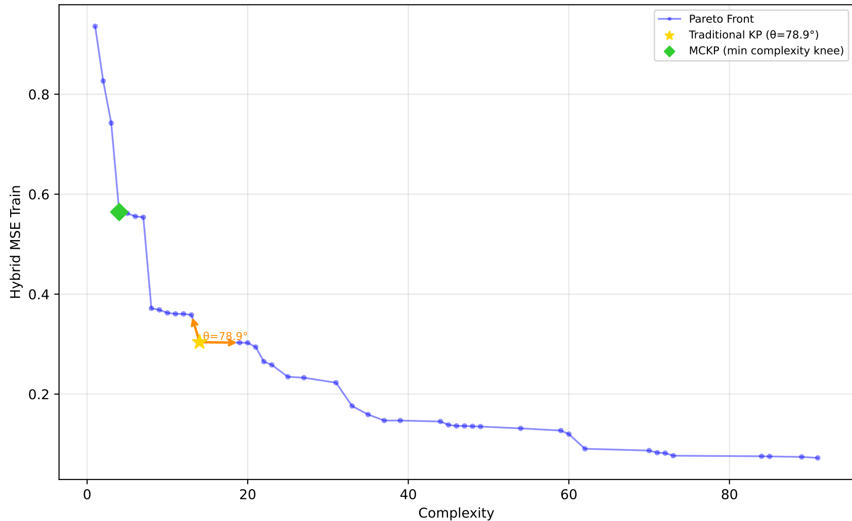
584_fri_c4_500_25 - Run 2 - MVP - Hybrid MSE Train \lambda_1=0.00, \lambda_2=0.00, \lambda_3=0.00 | Difficulty: 1.00 | Method: hmr
