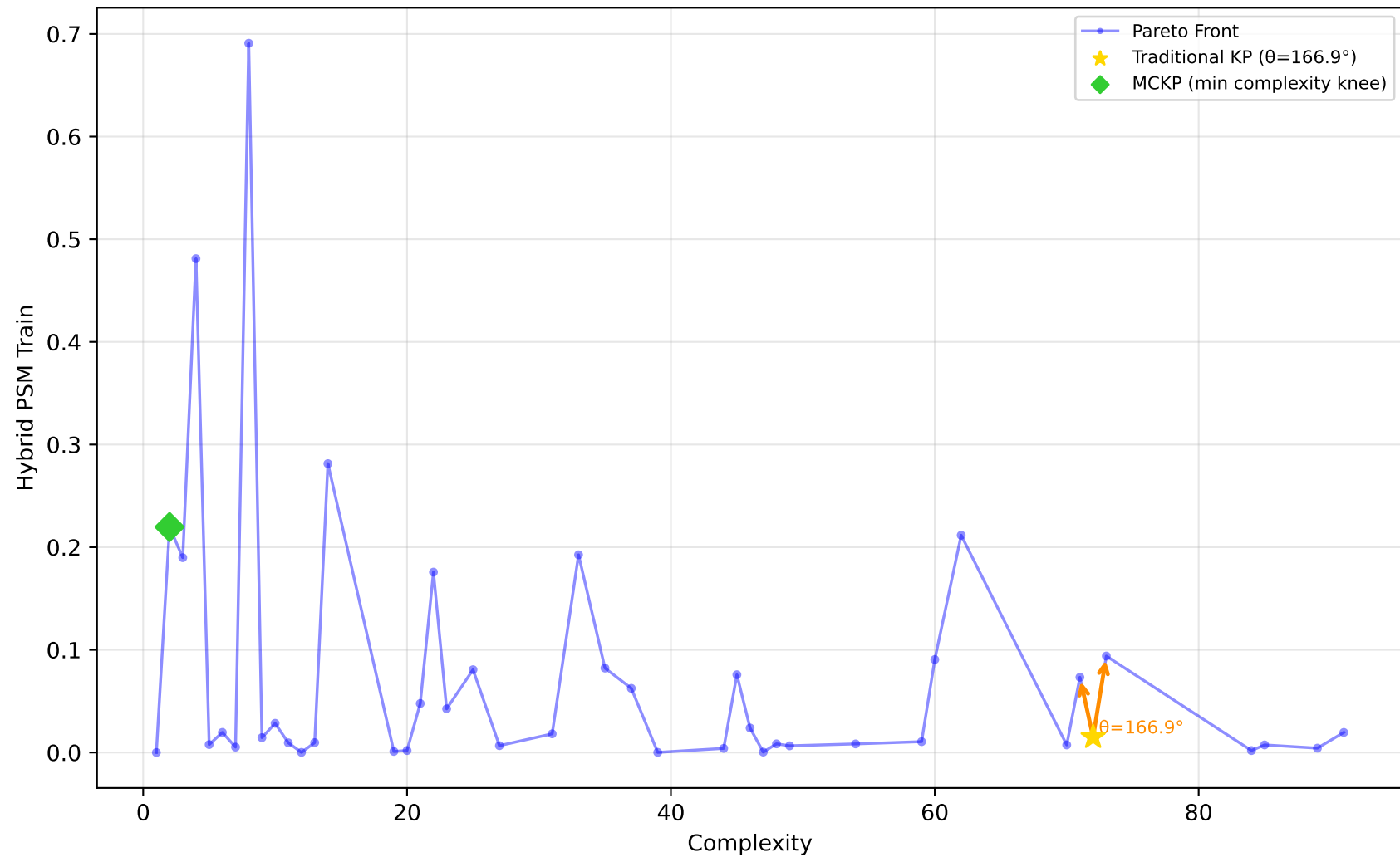
584_fri_c4_500_25 - Run 2 - MVP - Hybrid PSM Train \lambda_1=0.00, \lambda_2=0.00, \lambda_3=0.00 | Difficulty: 1.00 | Method: hmr
