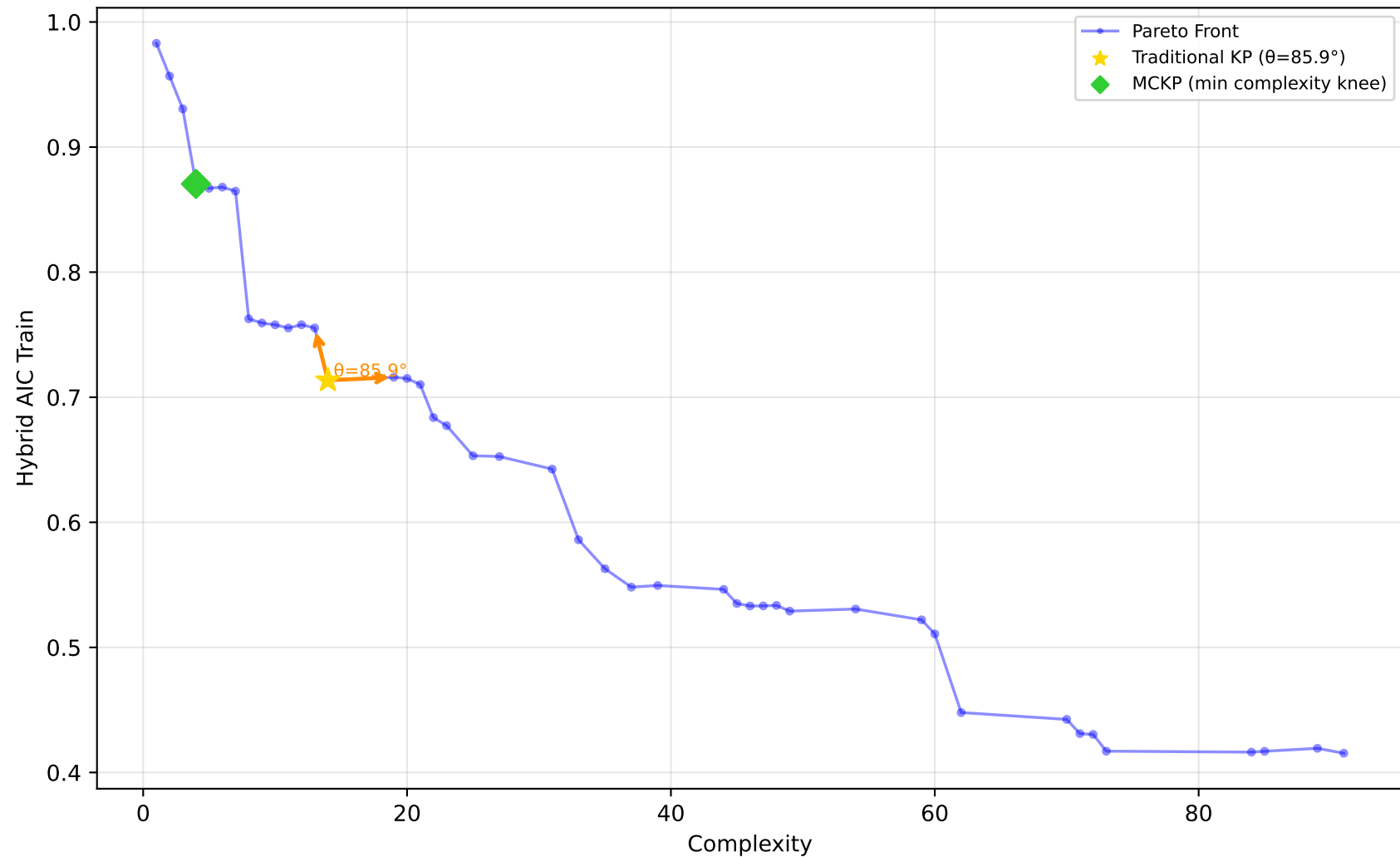
584_fri_c4_500_25 - Run 2 - SVP - Hybrid AIC Train \lambda_1=0.10, \lambda_2=0.40, \lambda_3=0.00 | Difficulty: 1.00 | Method: hmr
