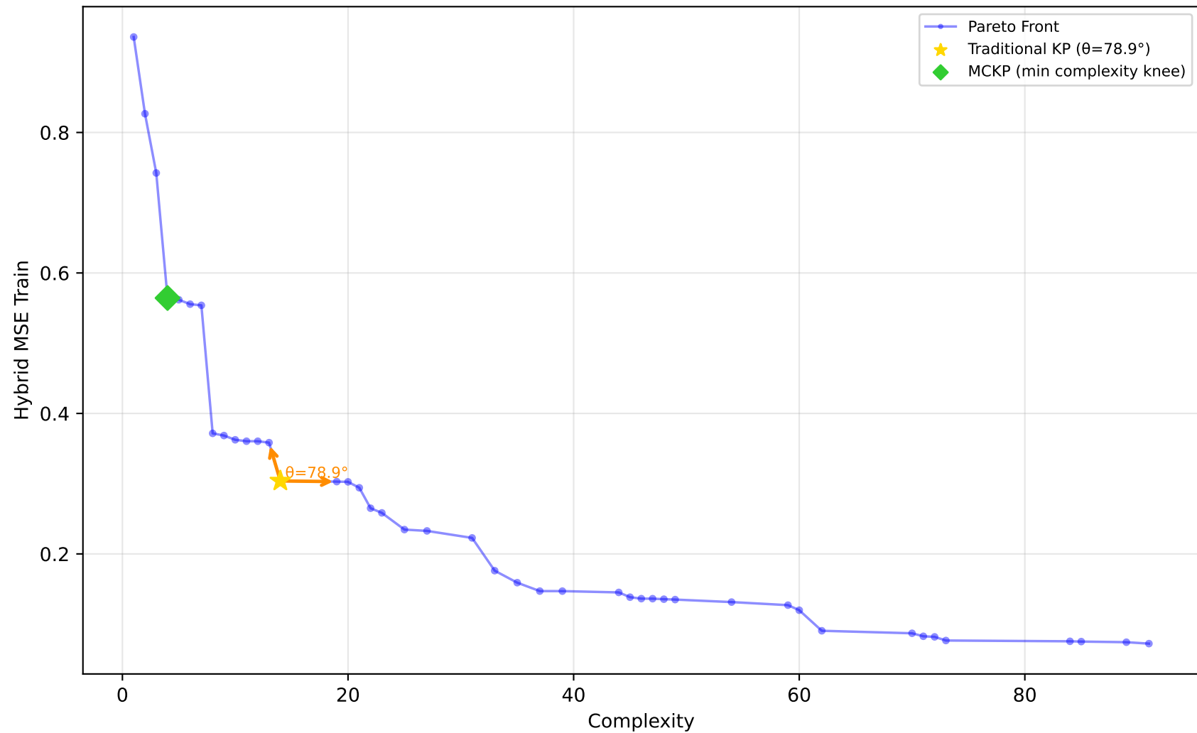
584_fri_c4_500_25 - Run 2 - SVP - Hybrid MSE Train \lambda_1=0.00, \lambda_2=0.00, \lambda_3=0.00 | Difficulty: 1.00 | Method: hmr
