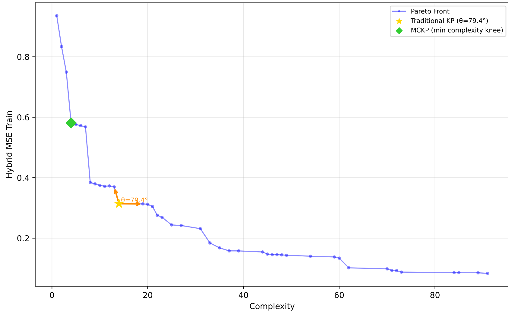
584_fri_c4_500_25 - Run 2 - SVP - Hybrid MSE Train \lambda_1=0.10, \lambda_2=0.40, \lambda_3=0.00 | Difficulty: 1.00 | Method: hmr
