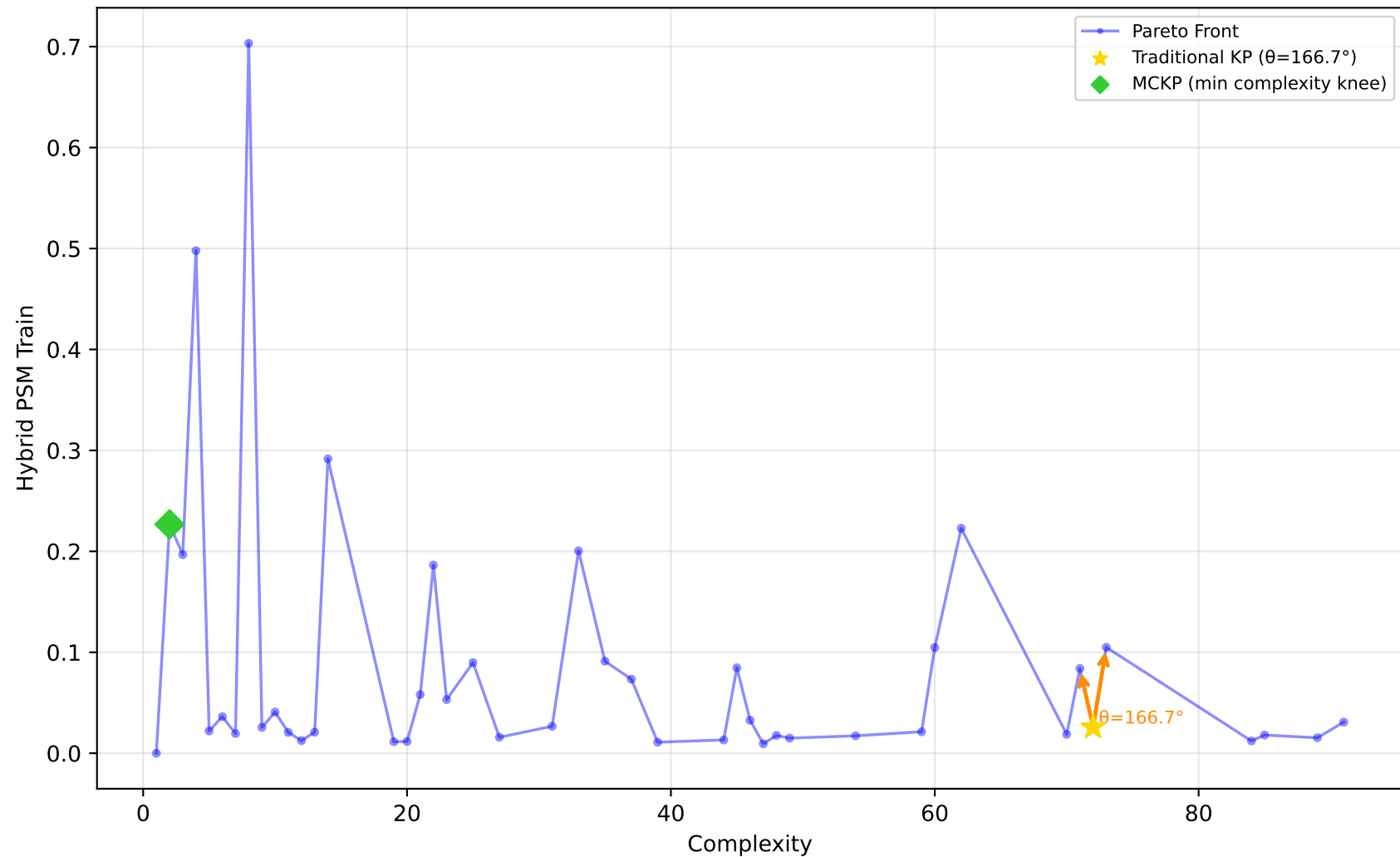
584_fri_c4_500_25 - Run 2 - SVP - Hybrid PSM Train \lambda_1=0.10, \lambda_2=0.40, \lambda_3=0.00 | Difficulty: 1.00 | Method: hmr
