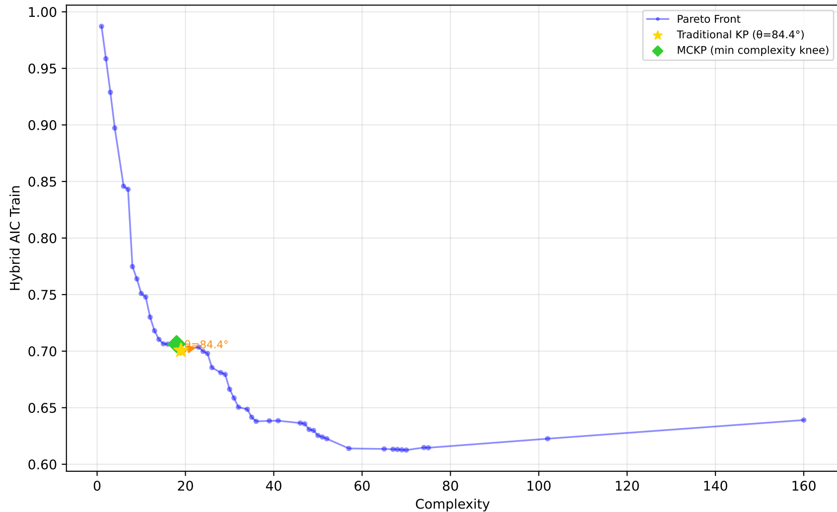
584_fri_c4_500_25 - Run 30 - MVP - Hybrid AIC Train \lambda_1=0.10, \lambda_2=0.00, \lambda_3=0.00 | Difficulty: 1.00 | Method: hmr
