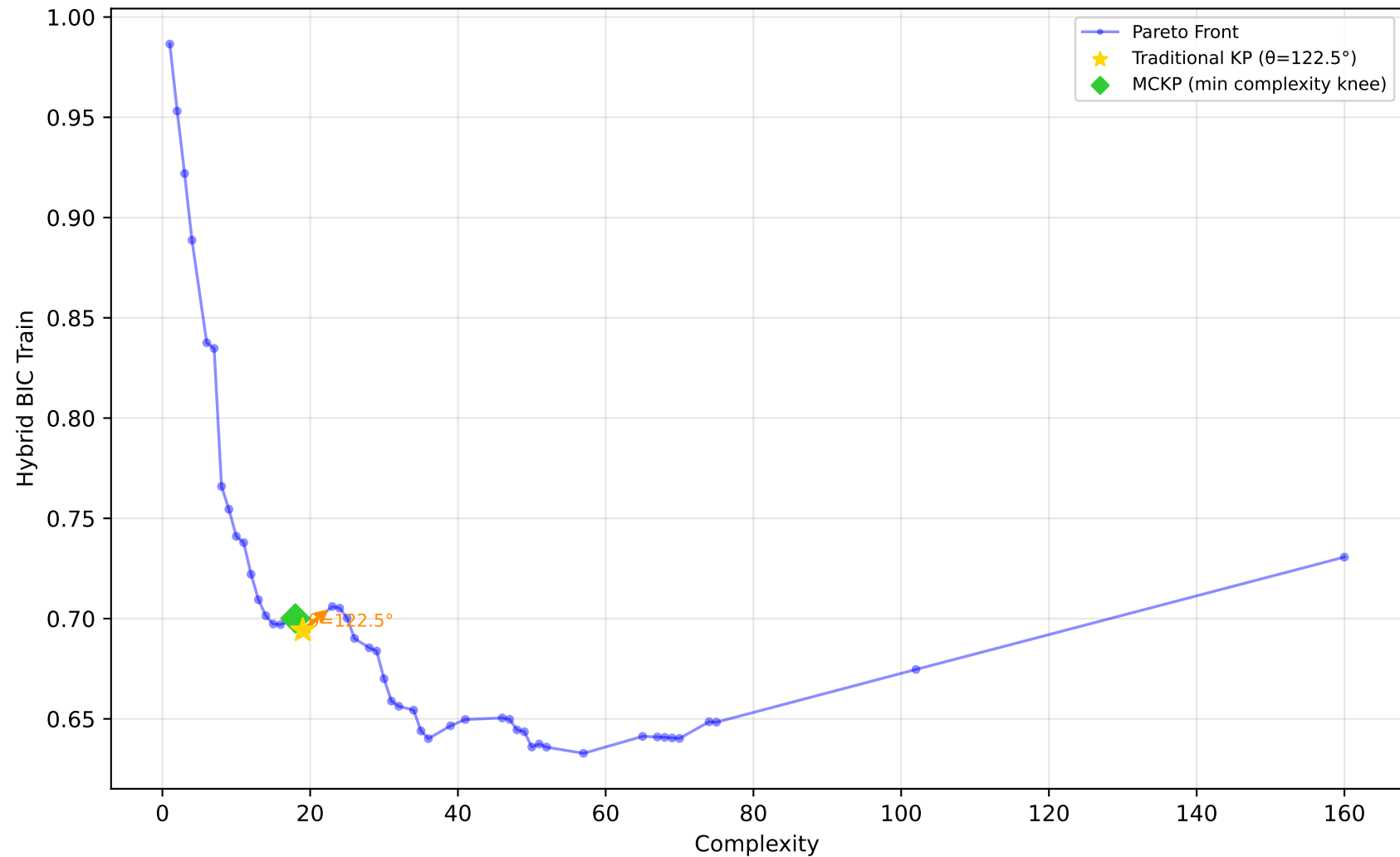
584_fri_c4_500_25 - Run 30 - MVP - Hybrid BIC Train \lambda_1=0.10, \lambda_2=0.00, \lambda_3=0.00 | Difficulty: 1.00 | Method: hmr
