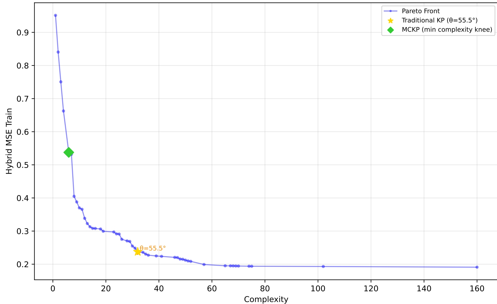
584_fri_c4_500_25 - Run 30 - MVP - Hybrid MSE Train \lambda_1=0.10, \bar{\lambda}_2=0.00, \bar{\lambda}_3=0.00 | Difficulty: 1.00 | Method: hmr
