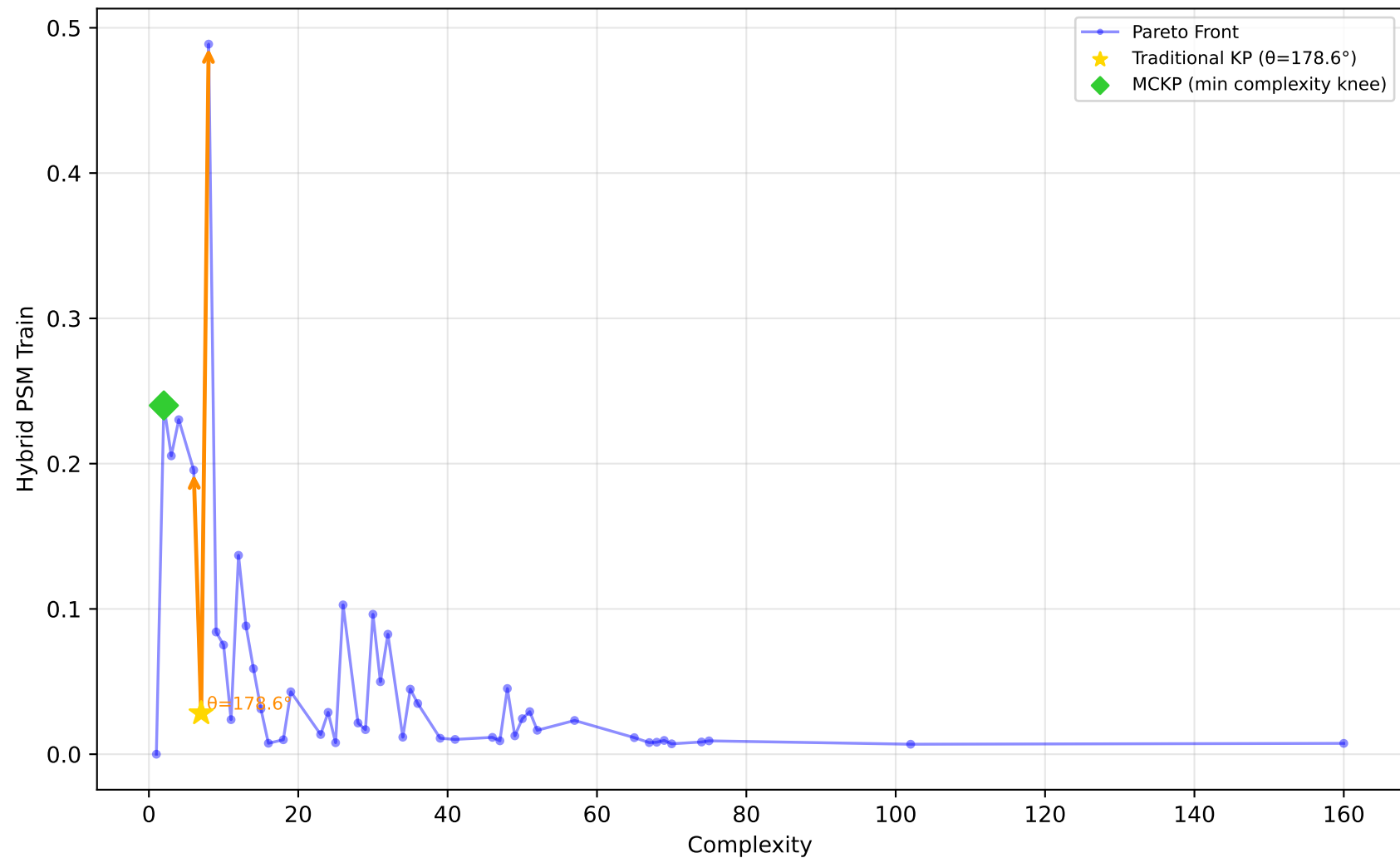
584_fri_c4_500_25 - Run 30 - MVP - Hybrid PSM Train \lambda_1=0.10, \bar{\lambda}_2=0.00, \bar{\lambda}_3=0.00 | Difficulty: 1.00 | Method: hmr
