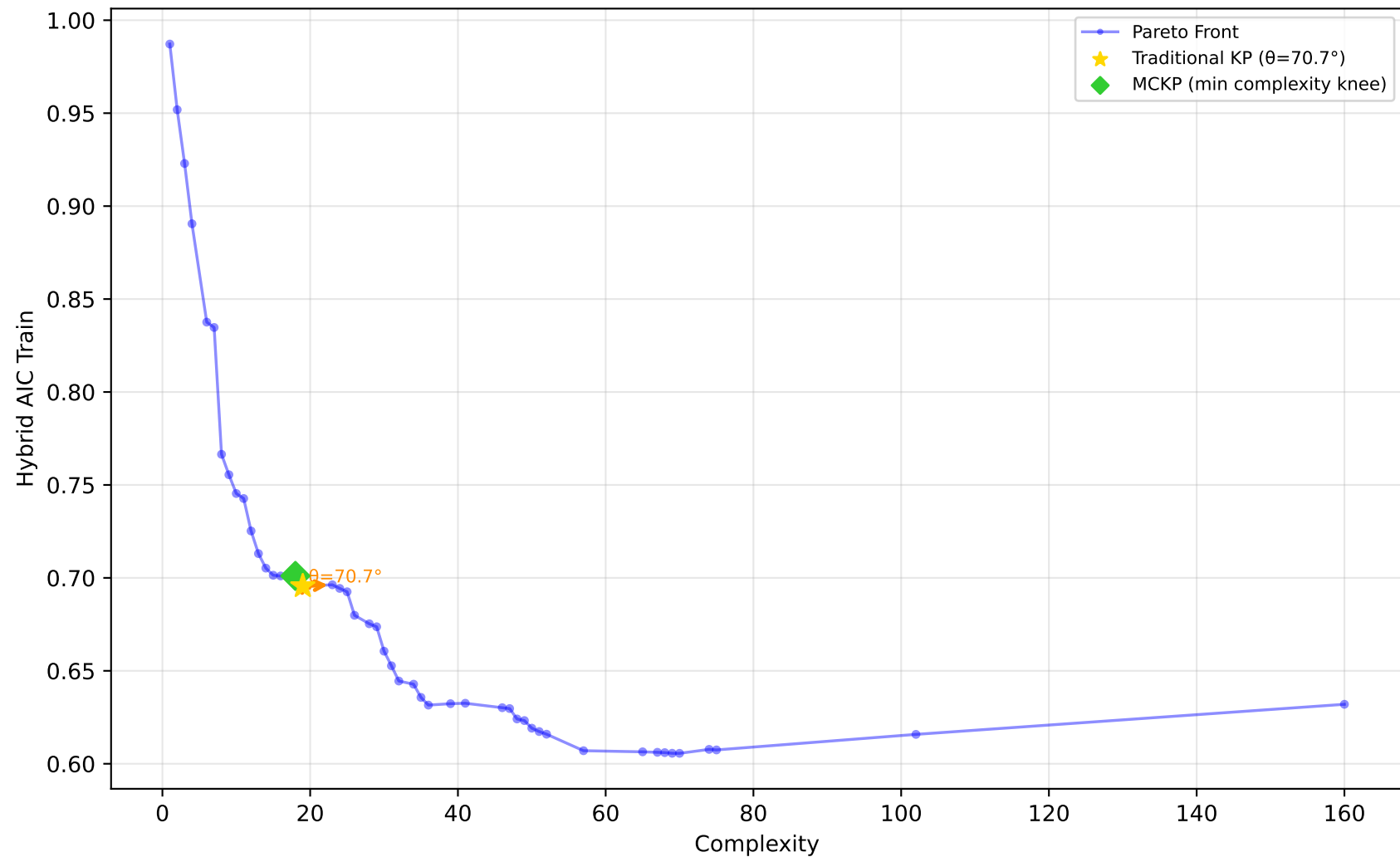
584_fri_c4_500_25 - Run 30 - SVP - Hybrid AIC Train \lambda_1=0.00, \lambda_2=0.00, \lambda_3=0.00 | Difficulty: 1.00 | Method: hmr
