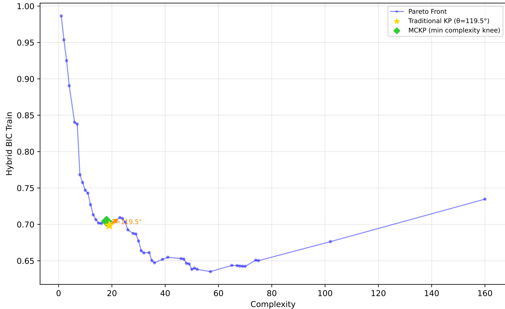
584_fri_c4_500_25 - Run 30 - SVP - Hybrid BIC Train \lambda_1=0.10, \lambda_2=0.40, \lambda_3=0.00 | Difficulty: 1.00 | Method: hmr
