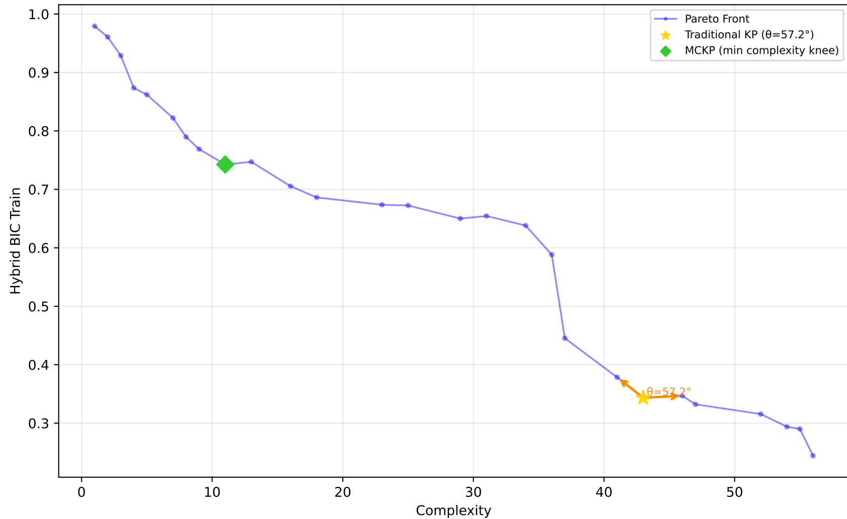
584_fri_c4_500_25 - Run 3 - MVP - Hybrid BIC Train \lambda_1=0.10, \lambda_2=0.00, \lambda_3=0.00 | Difficulty: 1.00 | Method: hmr
