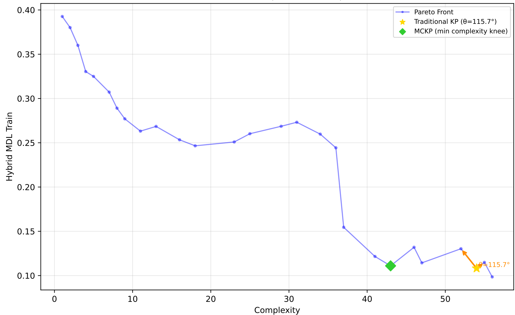
584_fri_c4_500_25 - Run 3 - MVP - Hybrid MDL Train \lambda_1=0.00, \lambda_2=0.00, \lambda_3=0.00 | Difficulty: 1.00 | Method: hmr
