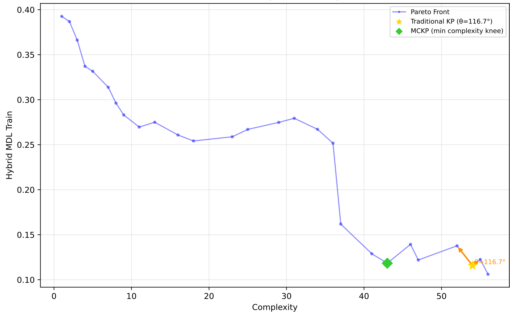
584_fri_c4_500_25 - Run 3 - MVP - Hybrid MDL Train \lambda_1=0.10, \lambda_2=0.00, \lambda_3=0.00 | Difficulty: 1.00 | Method: hmr
