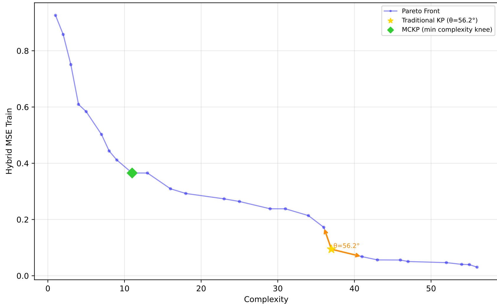
584_fri_c4_500_25 - Run 3 - MVP - Hybrid MSE Train \lambda_1=0.00, \lambda_2=0.00, \lambda_3=0.00 | Difficulty: 1.00 | Method: hmr
