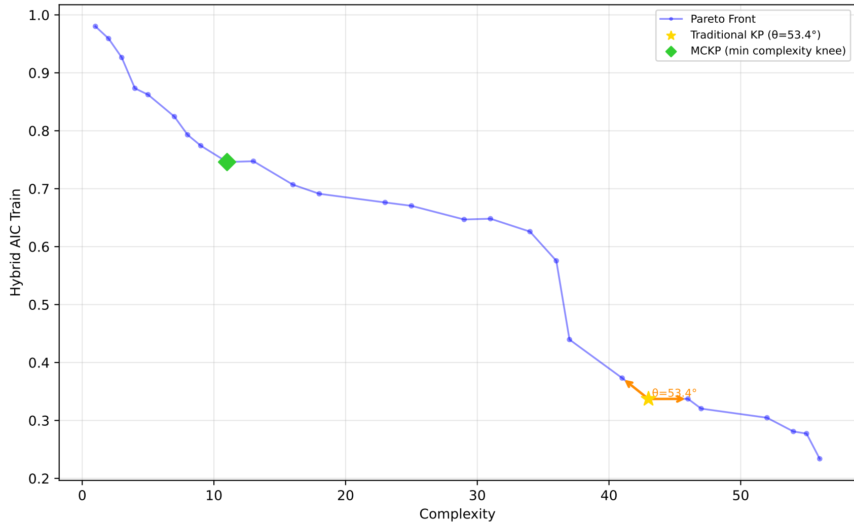
584_fri_c4_500_25 - Run 3 - SVP - Hybrid AIC Train \lambda_1=0.00, \lambda_2=0.00, \lambda_3=0.00 | Difficulty: 1.00 | Method: hmr
