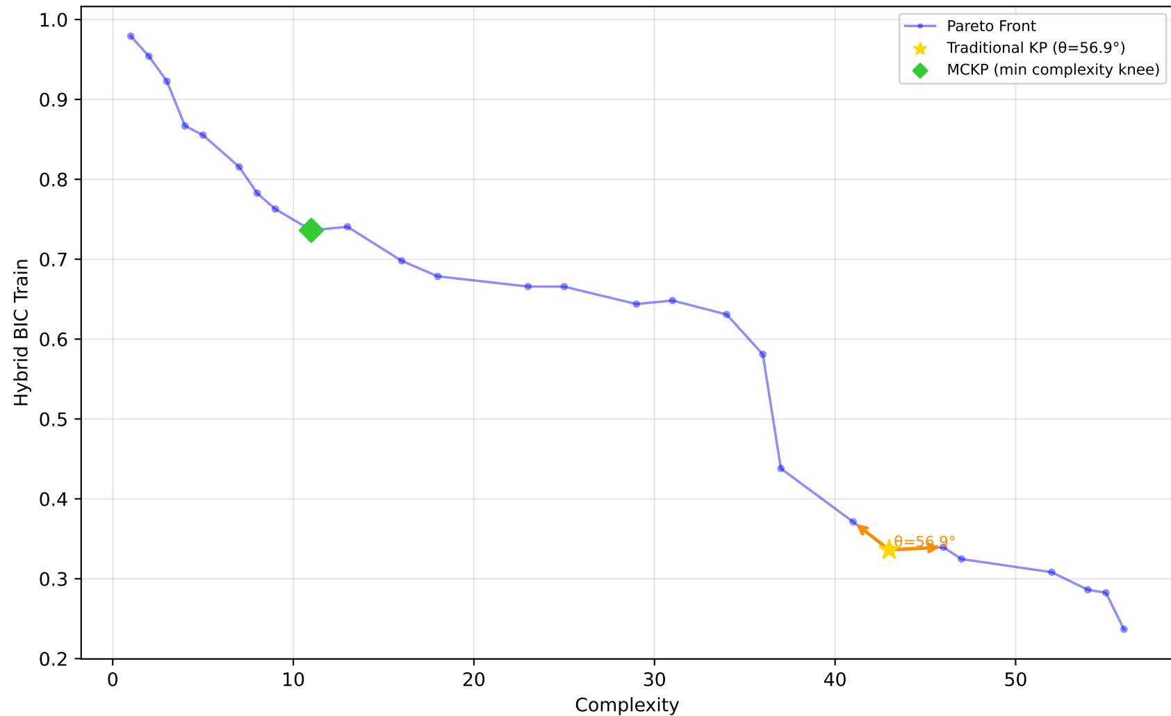
584_fri_c4_500_25 - Run 3 - SVP - Hybrid BIC Train \lambda_1=0.00, \lambda_2=0.00, \lambda_3=0.00 | Difficulty: 1.00 | Method: hmr
