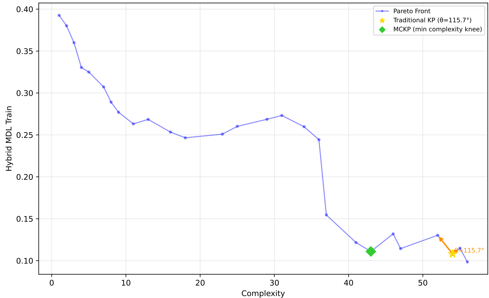
584_fri_c4_500_25 - Run 3 - SVP - Hybrid MDL Train \lambda_1=0.00, \lambda_2=0.00, \lambda_3=0.00 | Difficulty: 1.00 | Method: hmr
