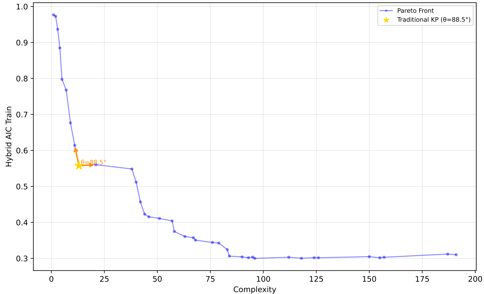
584_fri_c4_500_25 - Run 4 - MVP - Hybrid AIC Train \lambda_1=0.10, \lambda_2=0.00, \bar{\lambda}_3=0.00 | Difficulty: 1.00 | Method: hmr
