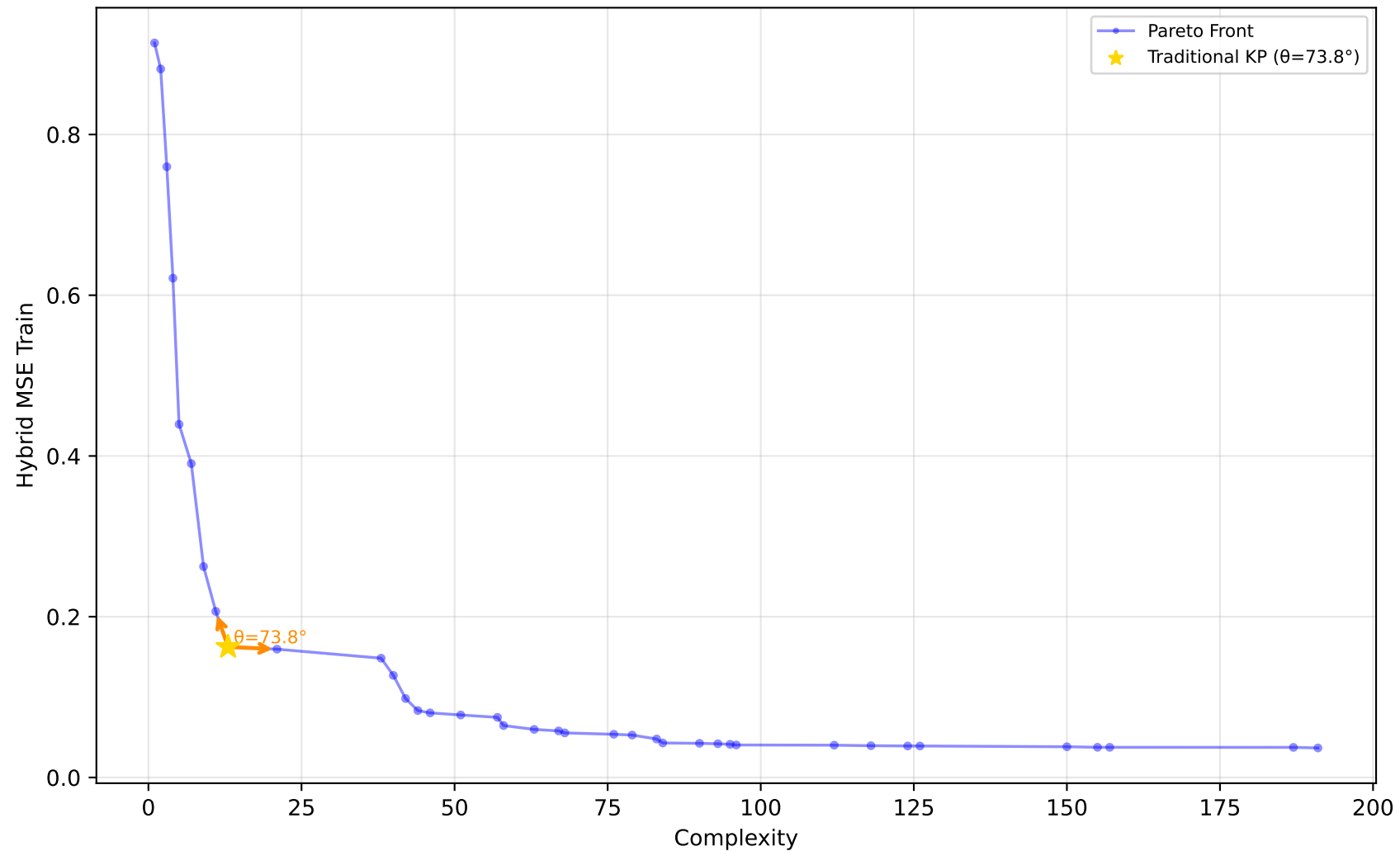
584_fri_c4_500_25 - Run 4 - MVP - Hybrid MSE Train \lambda_1=0.00, \lambda_2=0.00, \lambda_3=0.00 | Difficulty: 1.00 | Method: hmr
