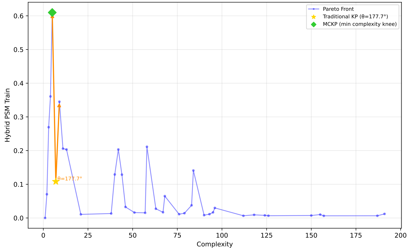
584_fri_c4_500_25 - Run 4 - MVP - Hybrid PSM Train \lambda_1=0.10, \lambda_2=0.00, \lambda_3=0.00 | Difficulty: 1.00 | Method: hmr
