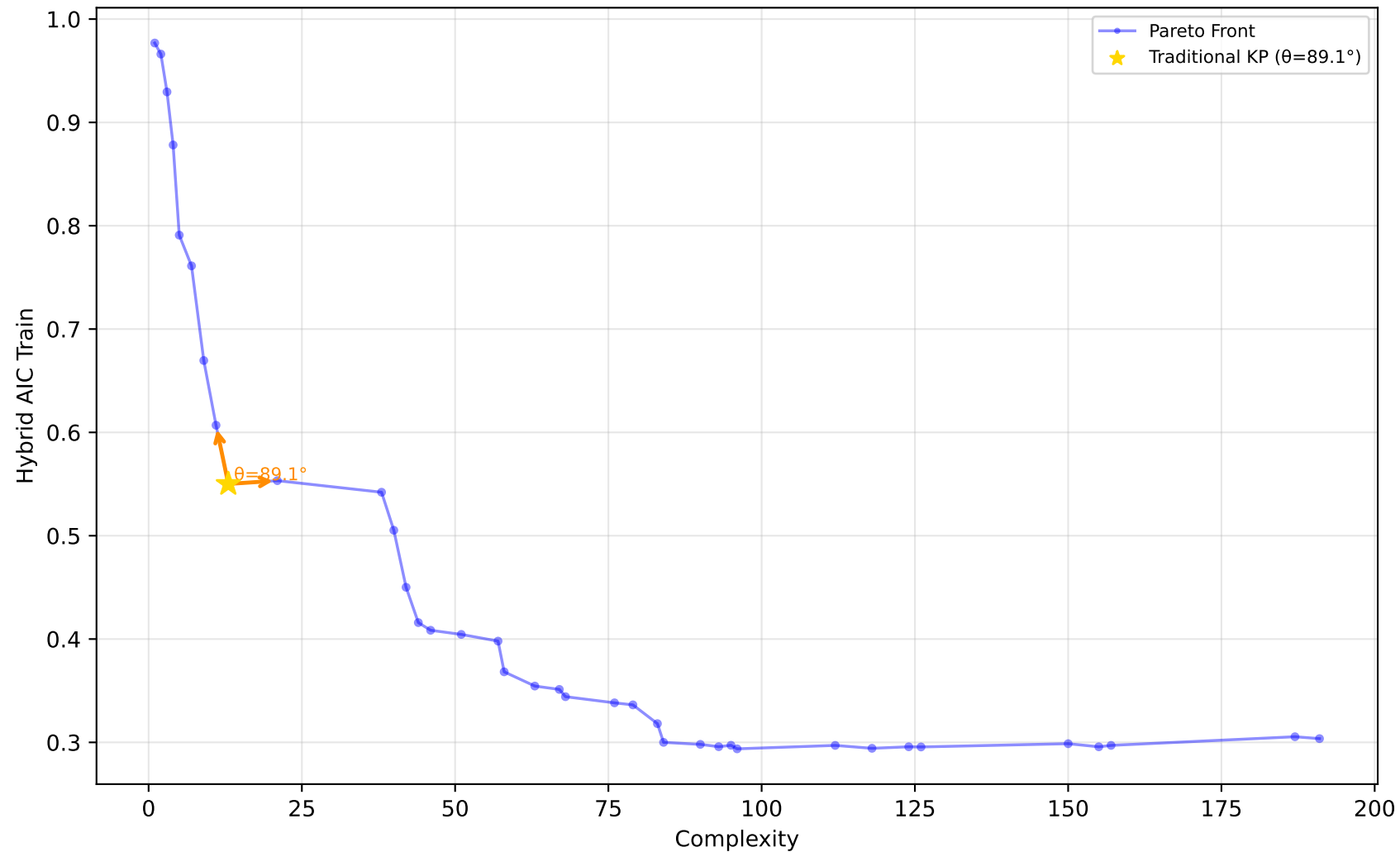
584_fri_c4_500_25 - Run 4 - SVP - Hybrid AIC Train \lambda_1=0.00, \lambda_2=0.00, \lambda_3=0.00 | Difficulty: 1.00 | Method: hmr
