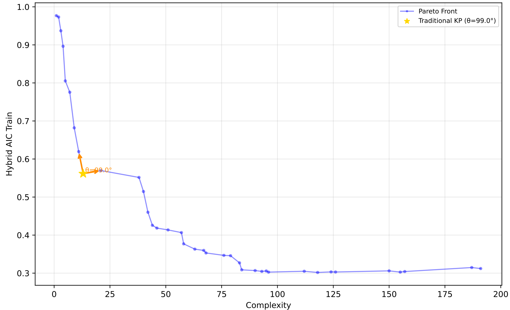
584_fri_c4_500_25 - Run 4 - SVP - Hybrid AIC Train \lambda_1=0.10, \lambda_2=0.40, \lambda_3=0.00 | Difficulty: 1.00 | Method: hmr
