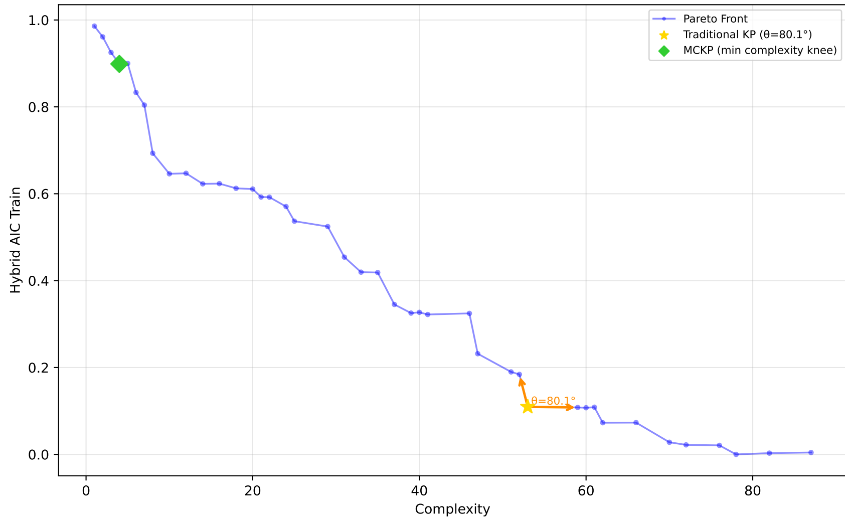
584_fri_c4_500_25 - Run 5 - MVP - Hybrid AIC Train \lambda_1=0.00, \lambda_2=0.00, \lambda_3=0.00 | Difficulty: 1.00 | Method: hmr
