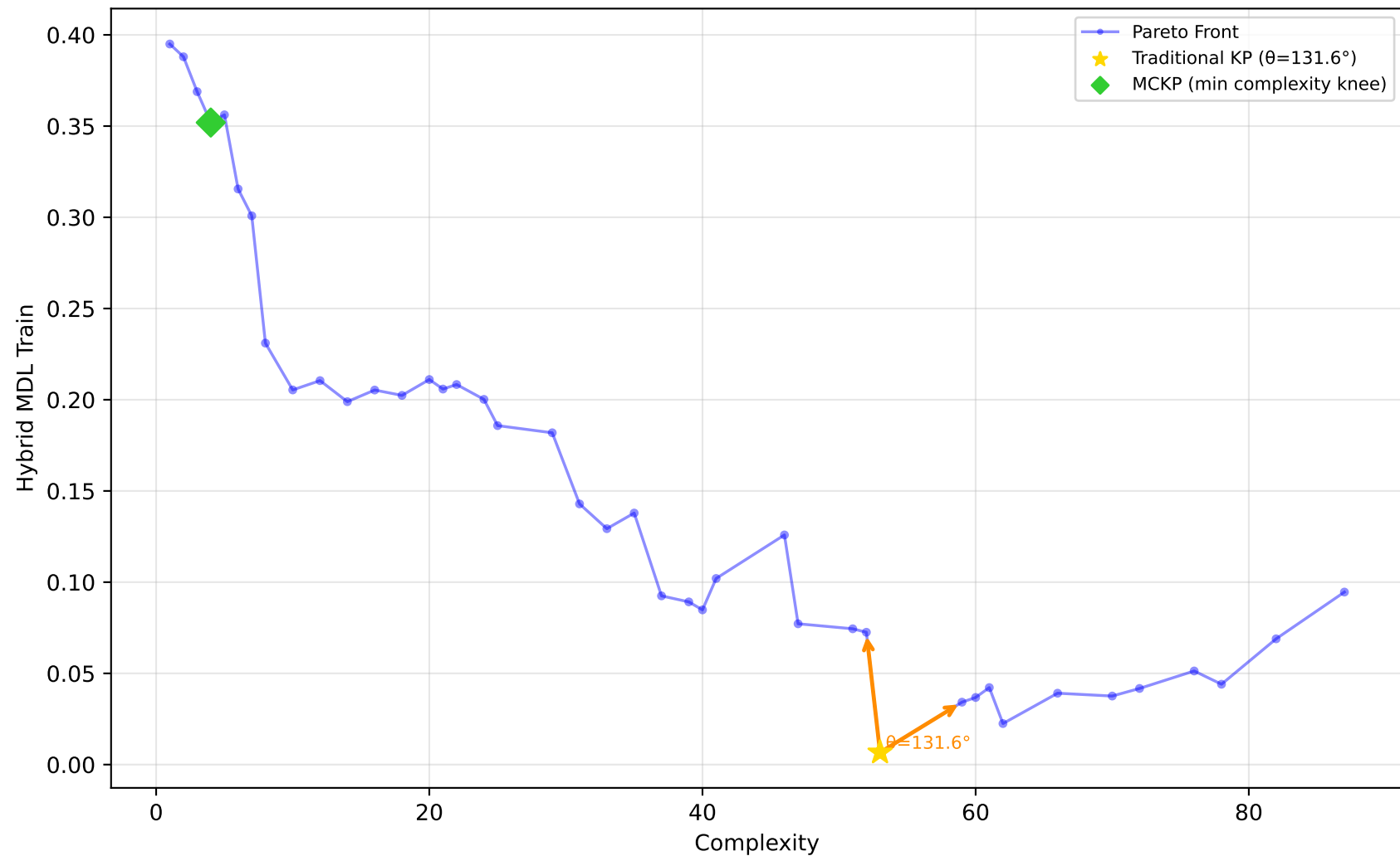
584_fri_c4_500_25 - Run 5 - MVP - Hybrid MDL Train \lambda_1=0.10, \lambda_2=0.00, \lambda_3=0.00 | Difficulty: 1.00 | Method: hmr
