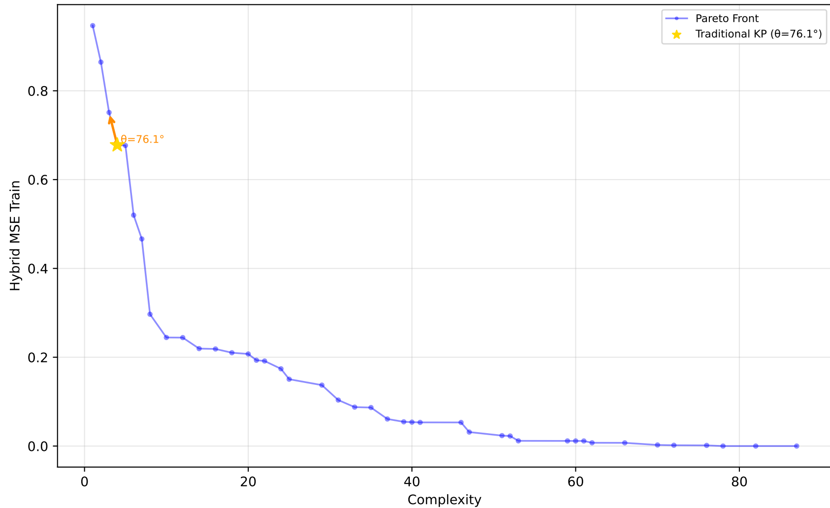
584_fri_c4_500_25 - Run 5 - MVP - Hybrid MSE Train \lambda_1=0.00, \lambda_2=0.00, \lambda_3=0.00 | Difficulty: 1.00 | Method: hmr
