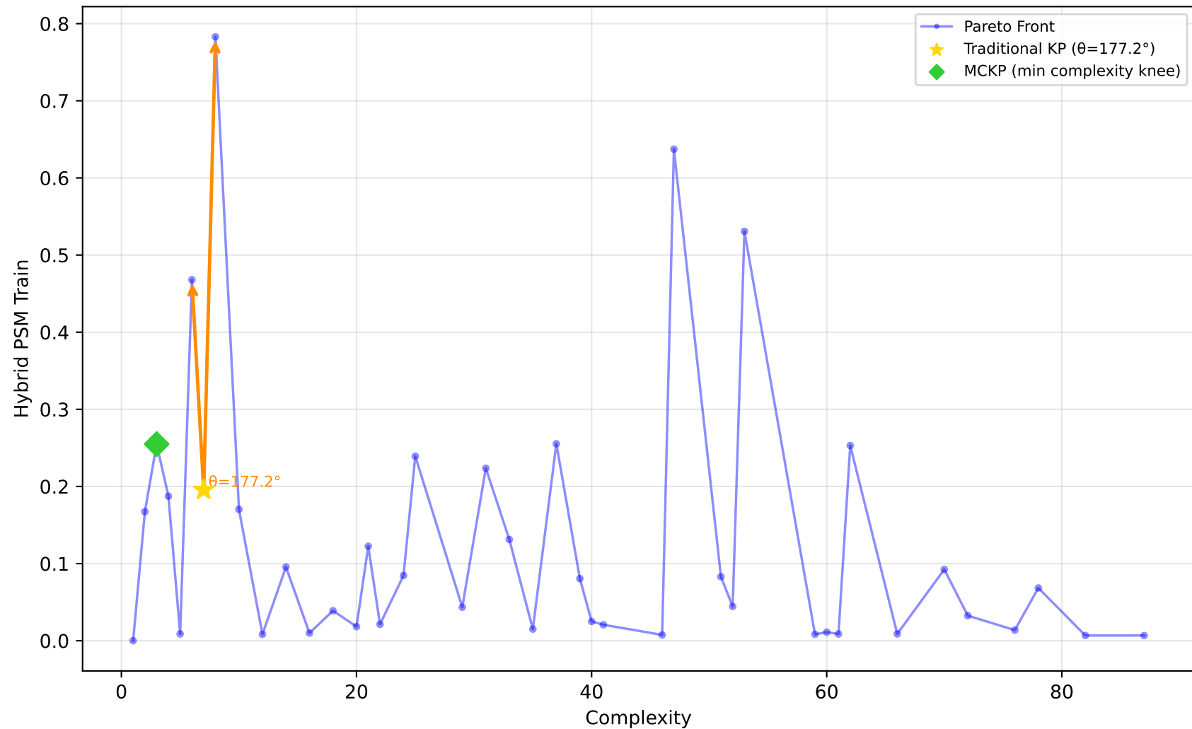
584_fri_c4_500_25 - Run 5 - MVP - Hybrid PSM Train \lambda_1=0.10, \lambda_2=0.00, \lambda_3=0.00 | Difficulty: 1.00 | Method: hmr
