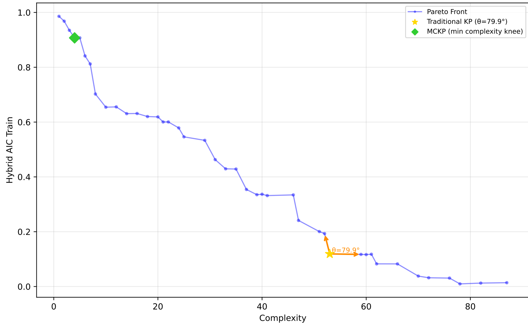
584_fri_c4_500_25 - Run 5 - SVP - Hybrid AIC Train \lambda_1=0.10, \lambda_2=0.40, \lambda_3=0.00 | Difficulty: 1.00 | Method: hmr
