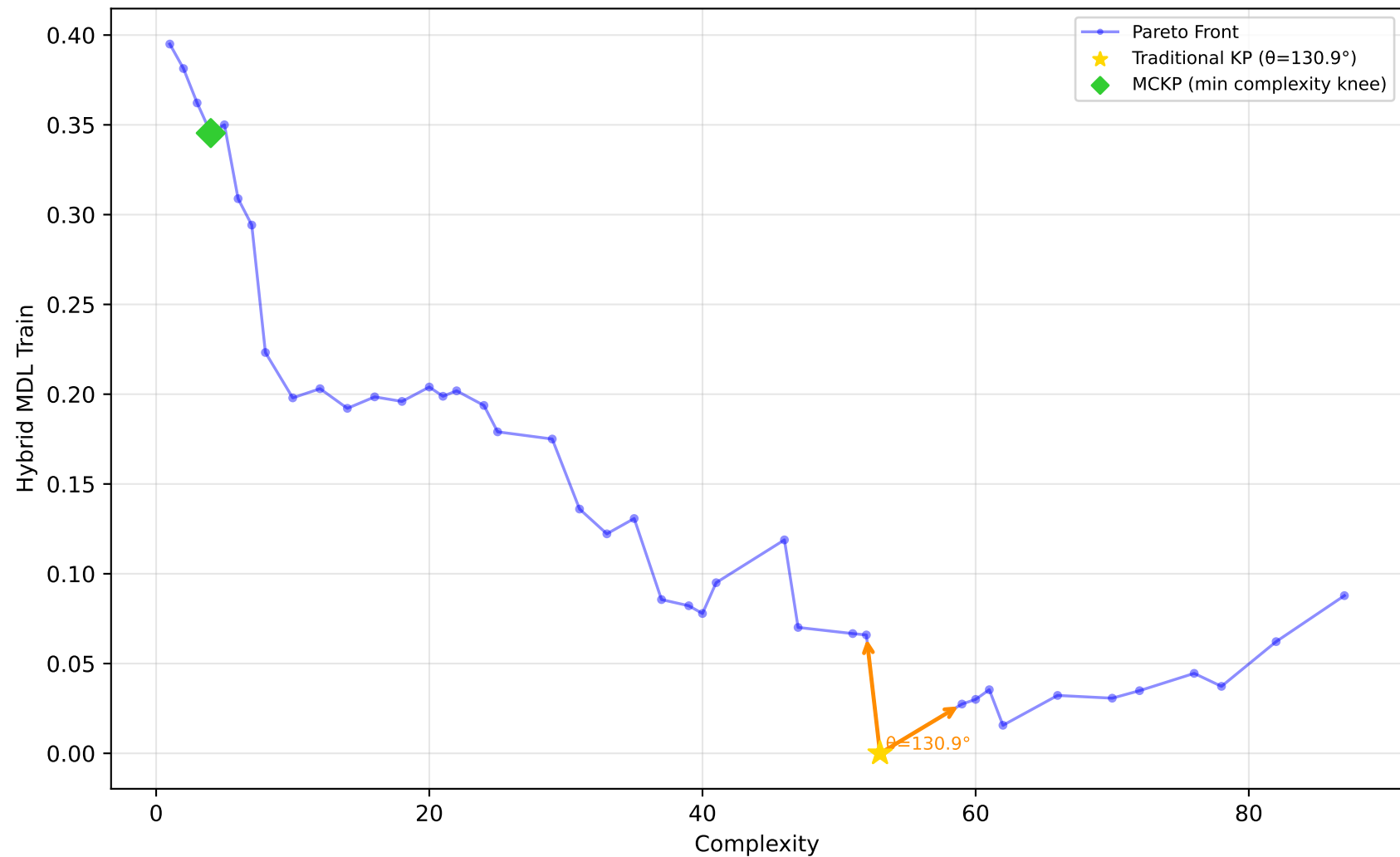
584_fri_c4_500_25 - Run 5 - SVP - Hybrid MDL Train \lambda_1=0.00 , \lambda_2=0.00 , \lambda_3=0.00 | Difficulty: 1.00 | Method: hmr
