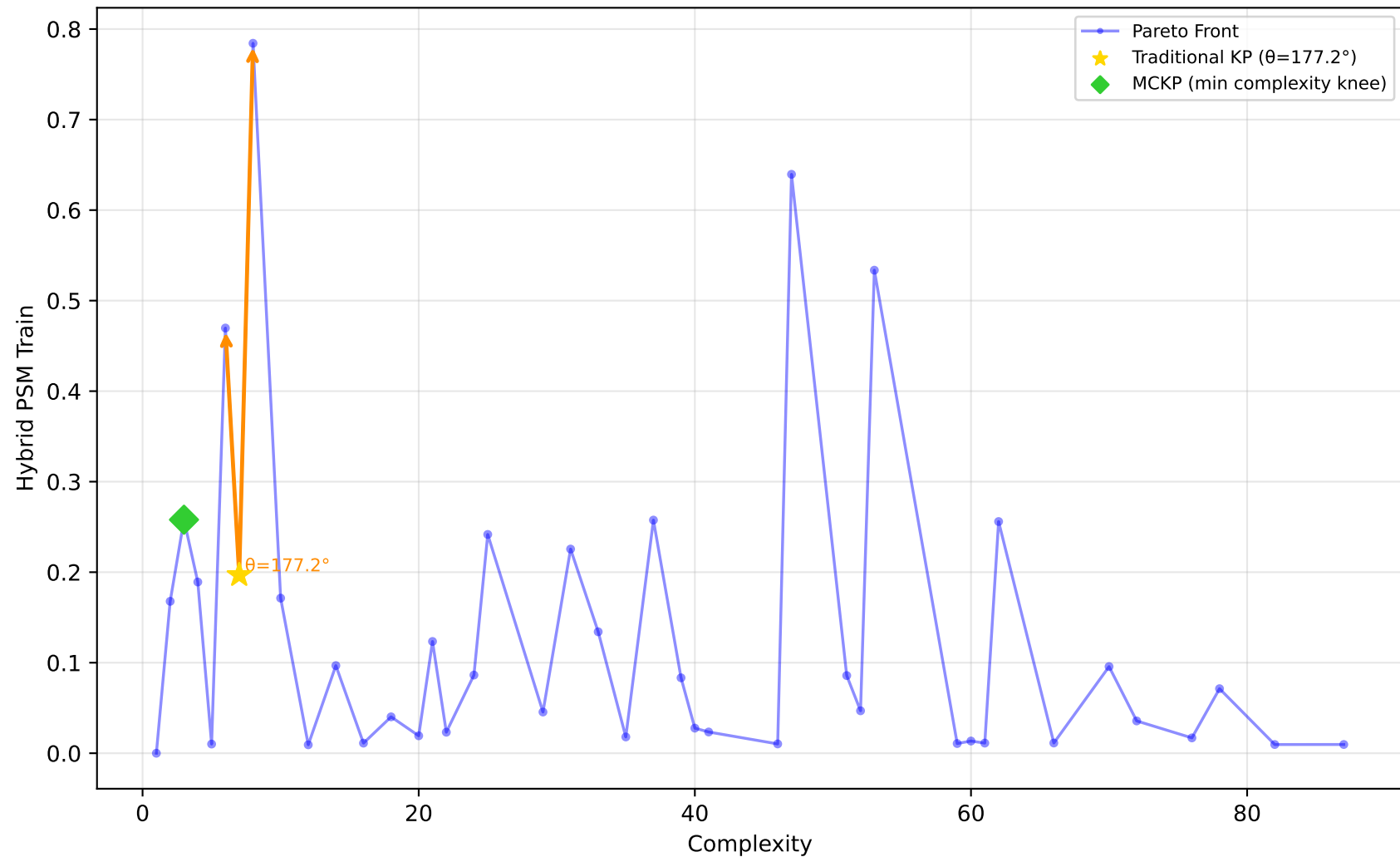
584_fri_c4_500_25 - Run 5 - SVP - Hybrid PSM Train \lambda_1=0.10, \lambda_2=0.40, \lambda_3=0.00 | Difficulty: 1.00 | Method: hmr
