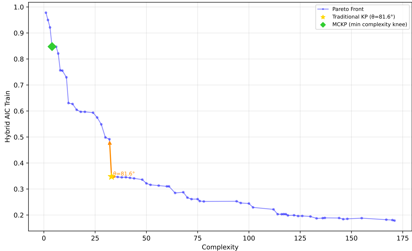
584_fri_c4_500_25 - Run 6 - MVP - Hybrid AIC Train \lambda_1=0.00, \lambda_2=0.00, \lambda_3=0.00 | Difficulty: 1.00 | Method: hmr
