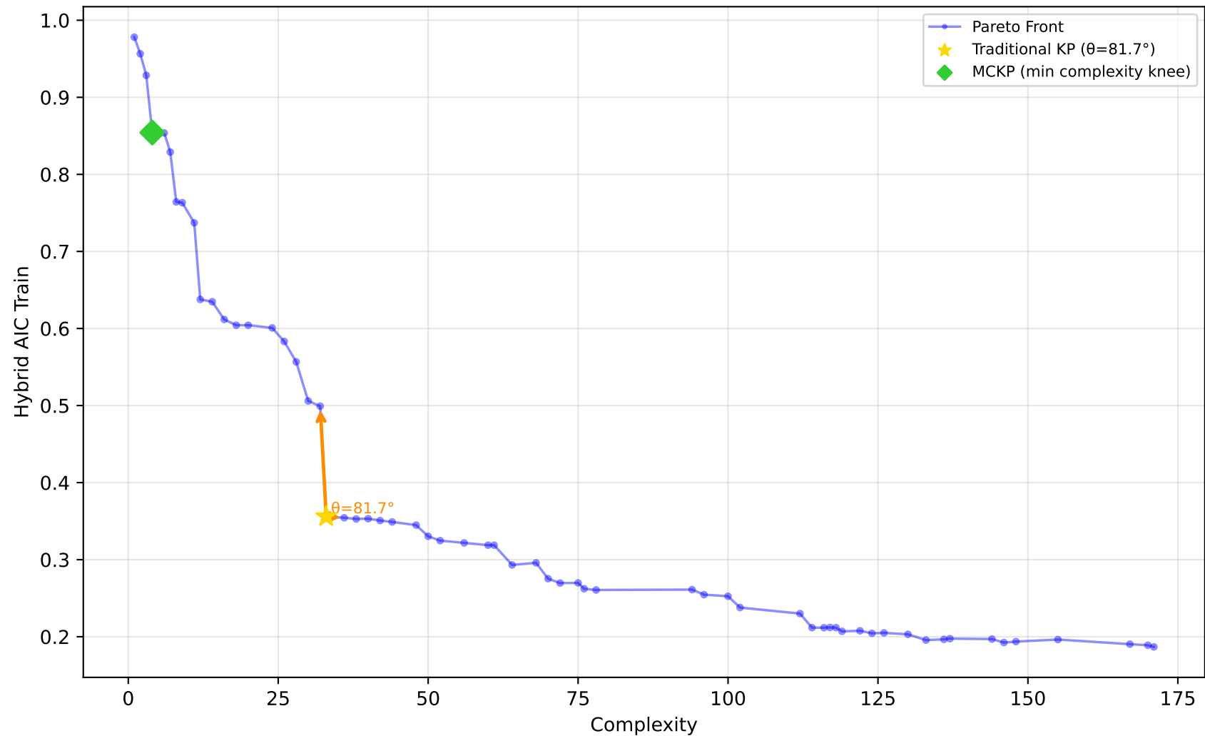
584_fri_c4_500_25 - Run 6 - MVP - Hybrid AIC Train \lambda_1=0.10, \lambda_2=0.00, \lambda_3=0.00 | Difficulty: 1.00 | Method: hmr
